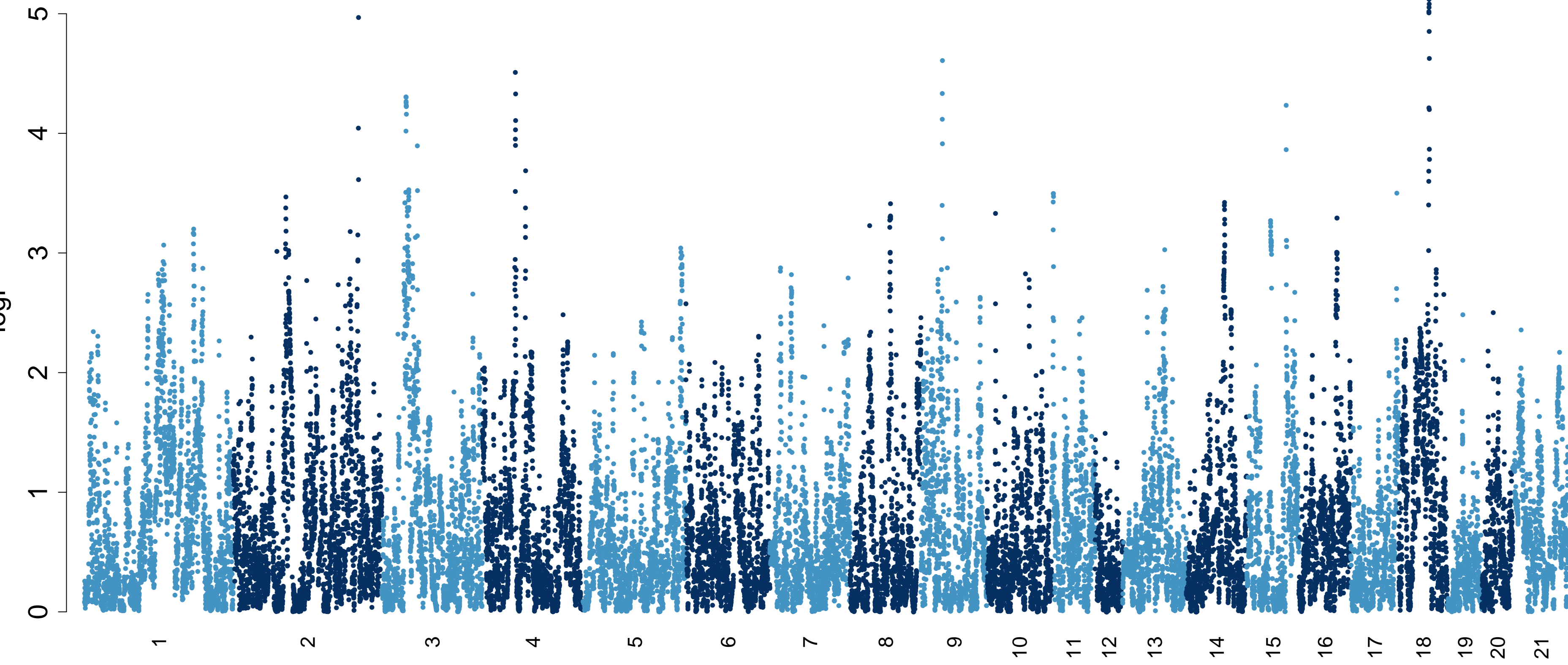
Activity_Distance15_20 imputed
