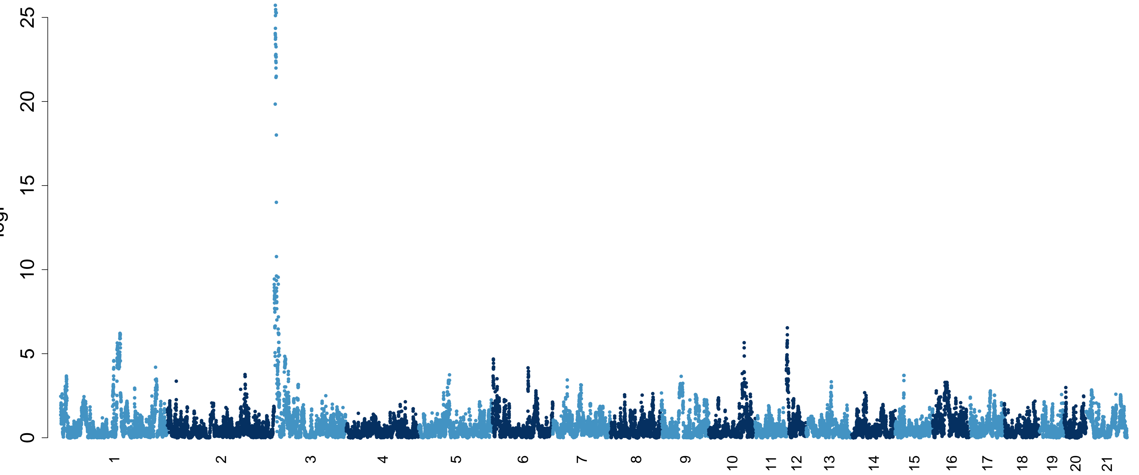
Biochemistry_ALP imputed
