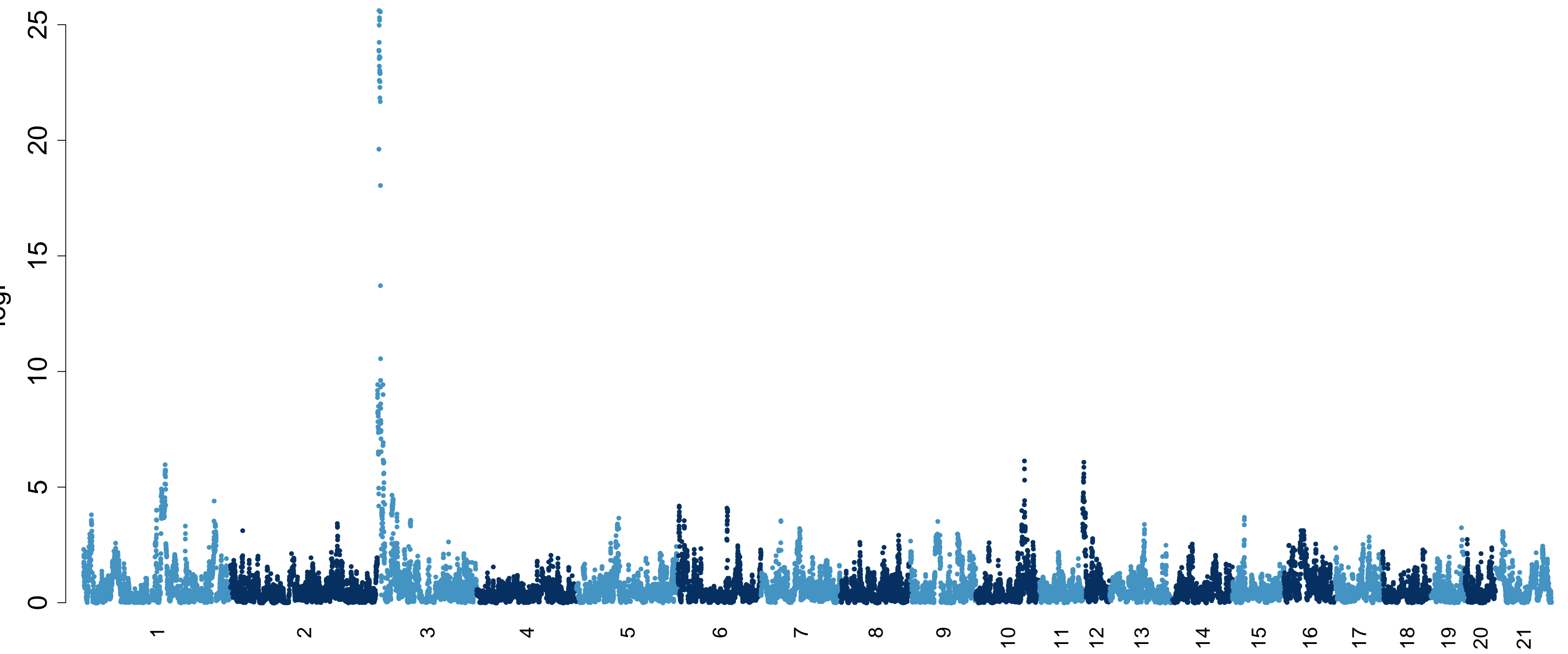
Biochemistry_ALP
