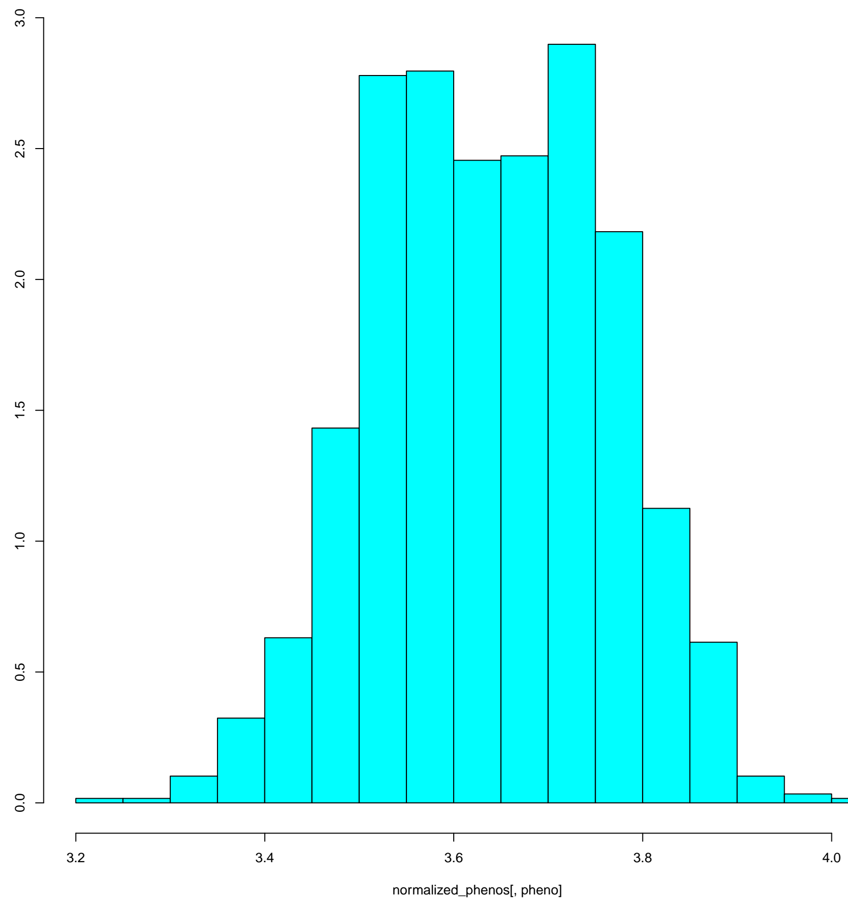
Normalized raw pheno
