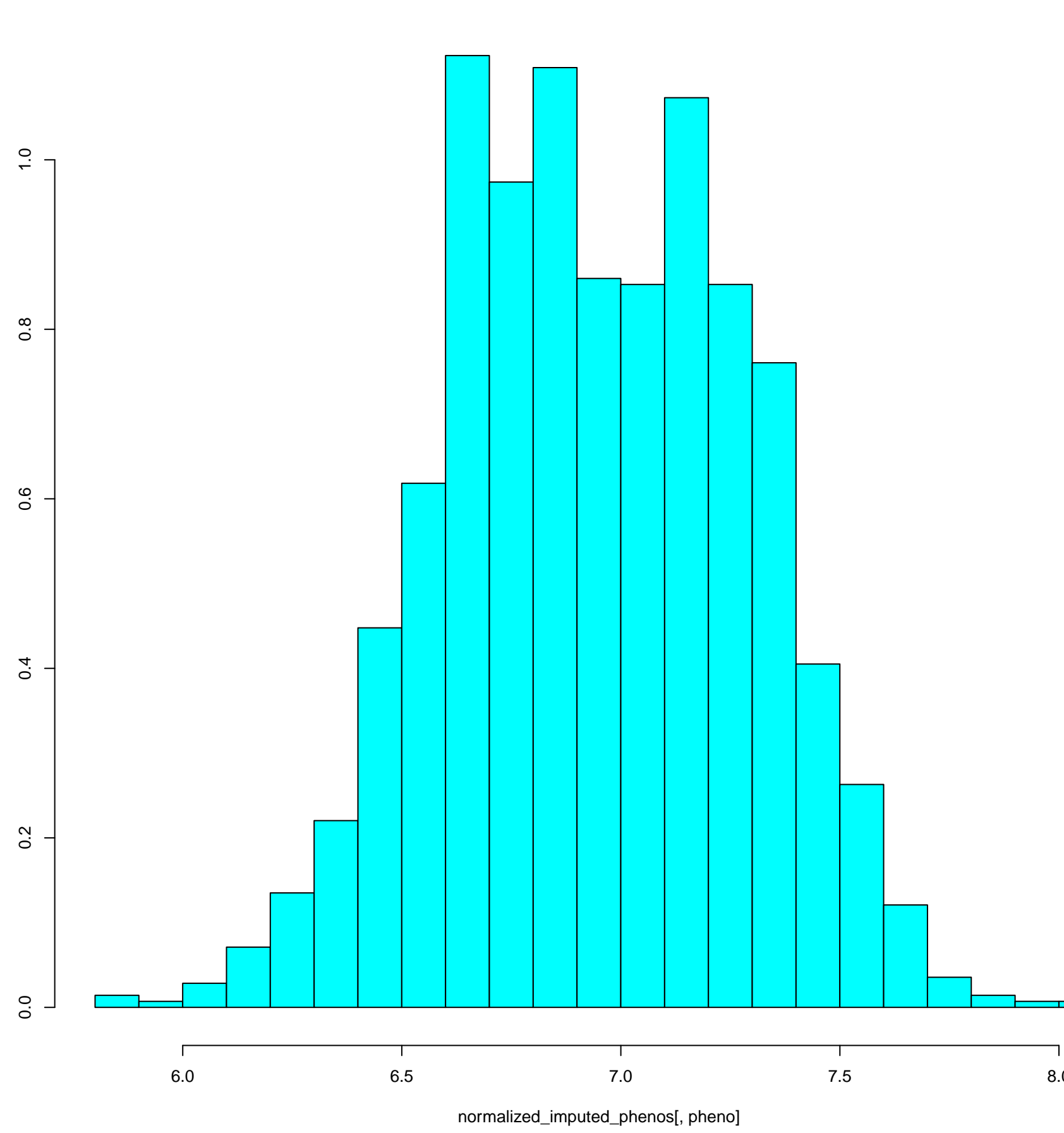
Normalized imputed pheno
