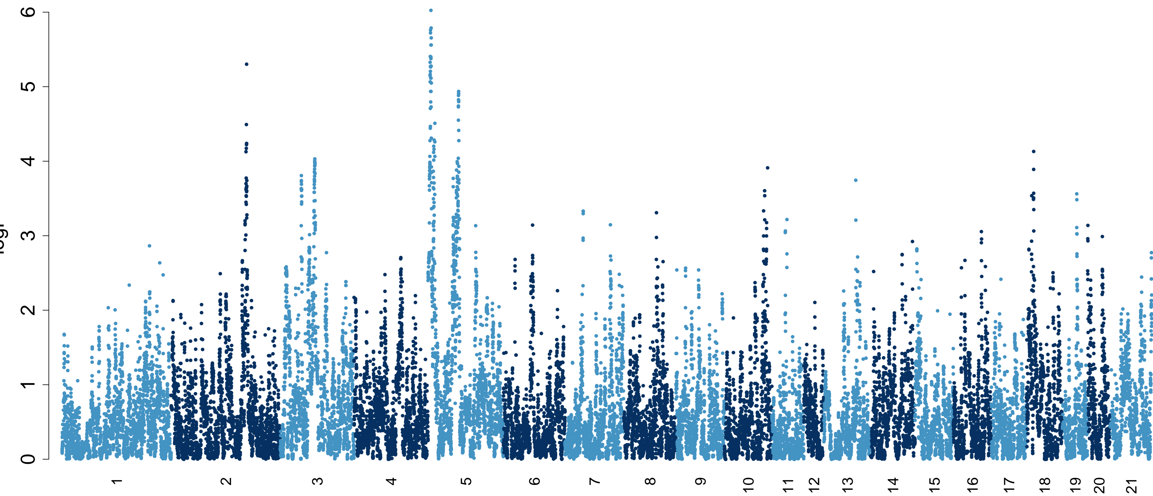
Bone_fem_neck_TOT_A imputed
