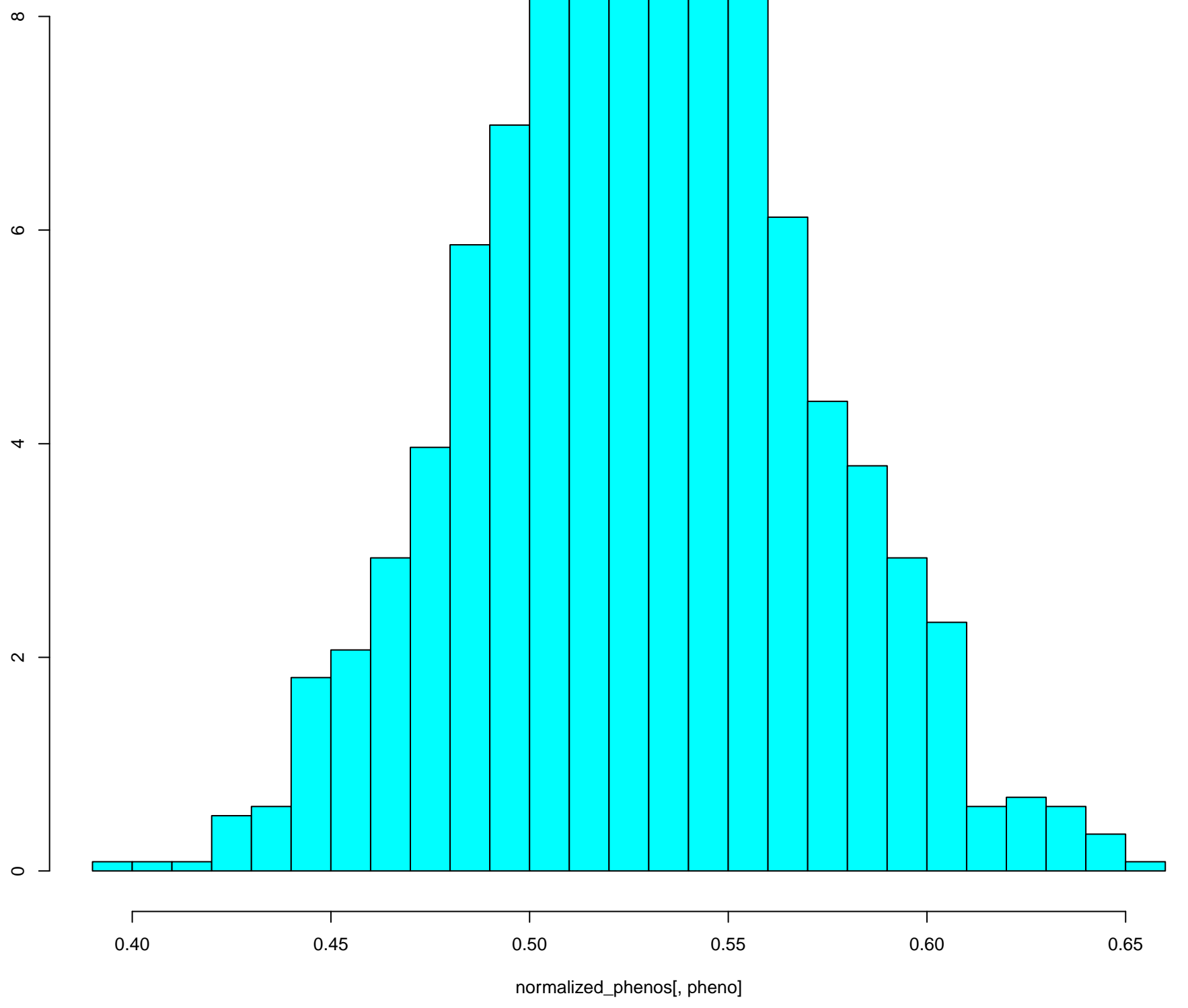
Normalized imputed pheno
