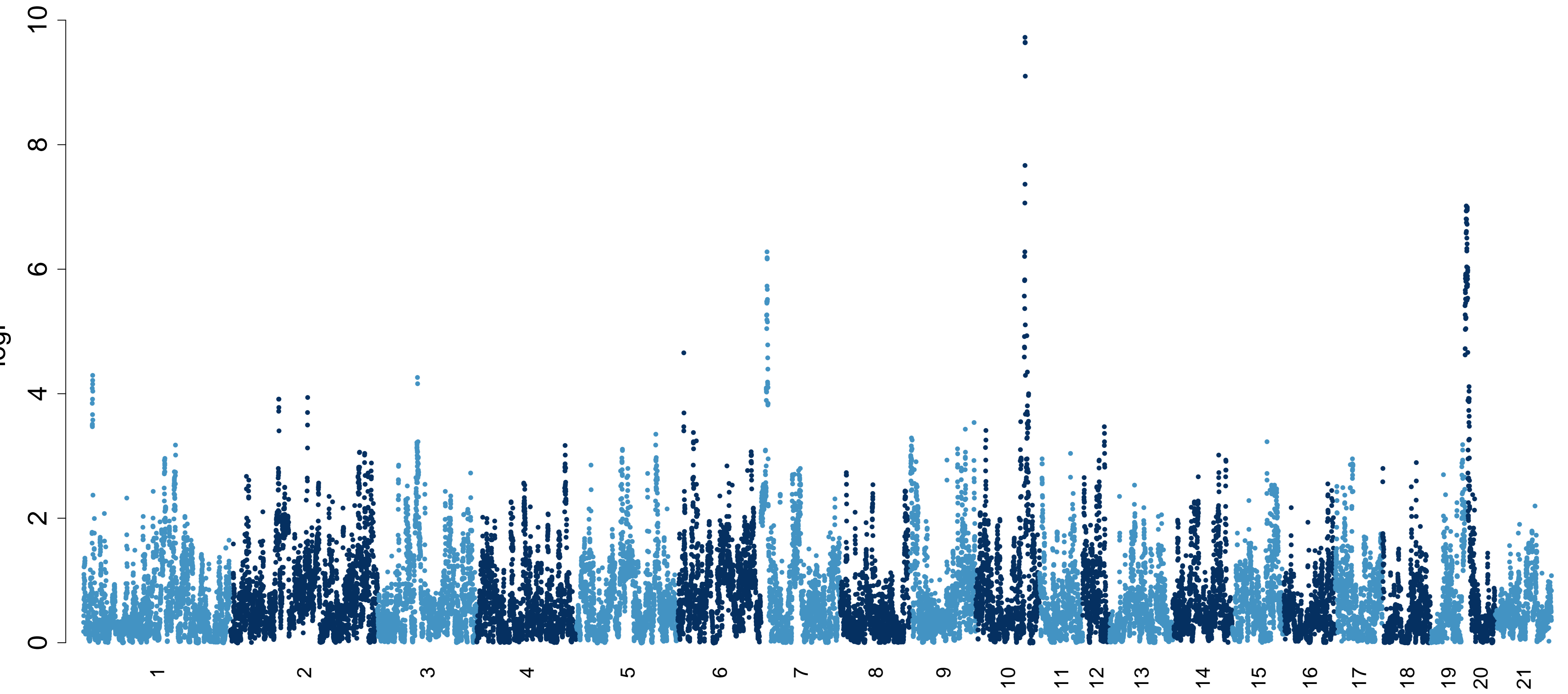
FACS_Abs_CD25CD8 imputed
