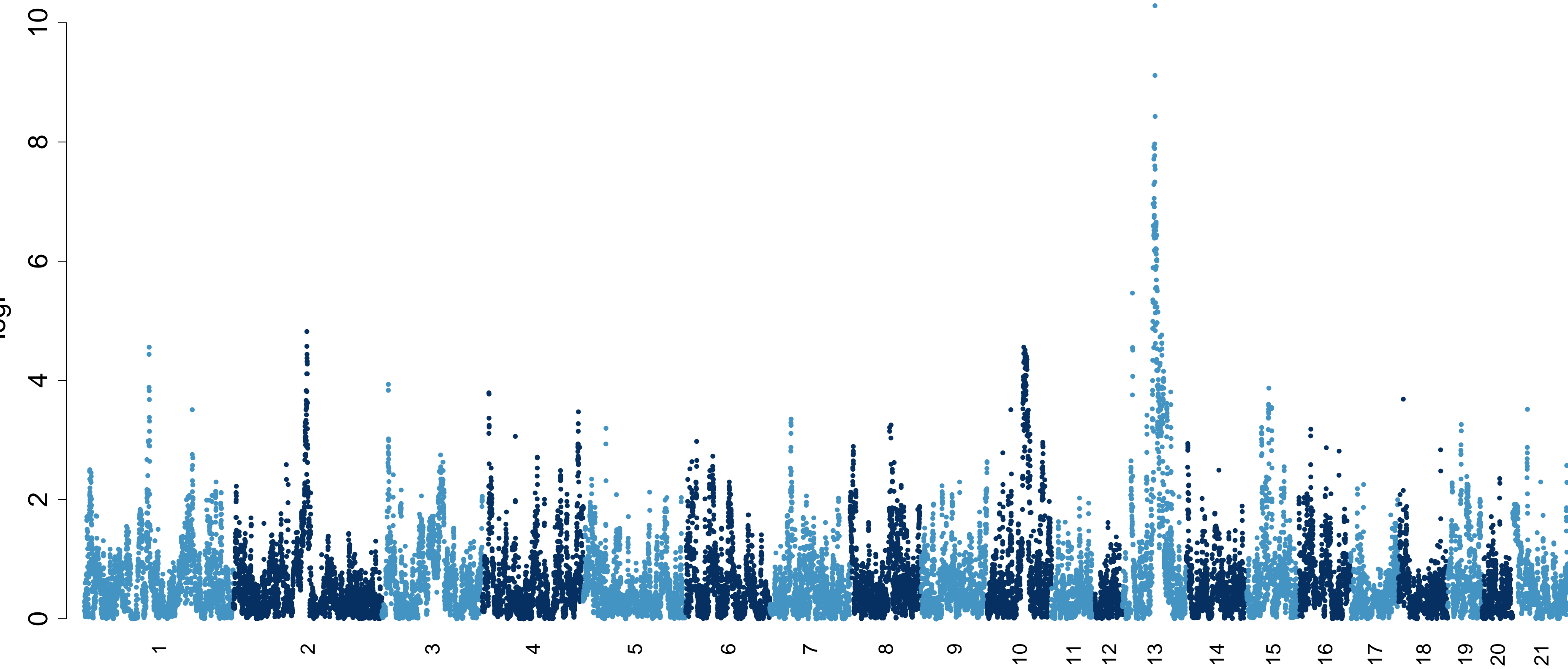
FACS_pctCD45RChighCD4
