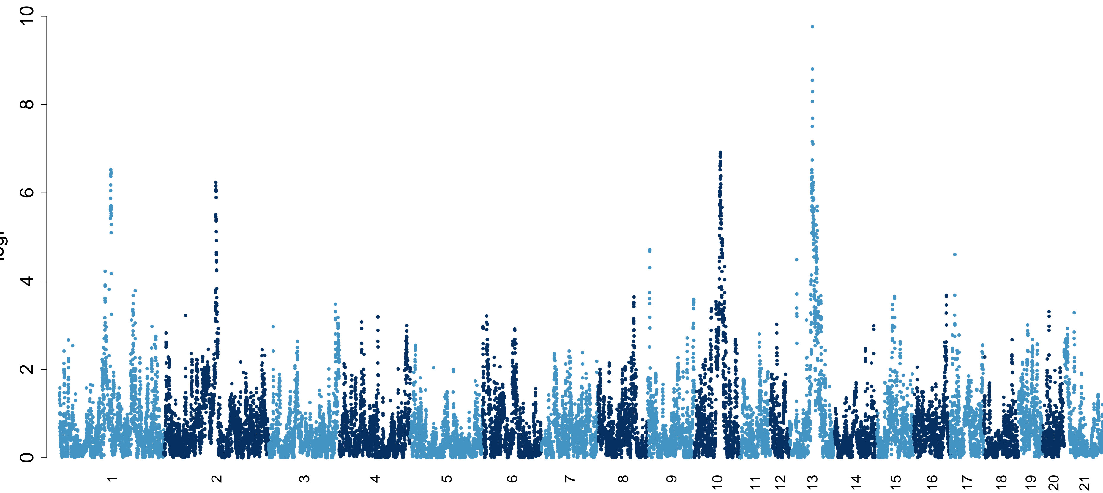
FACS_pctCD45RChighCD4 imputed
