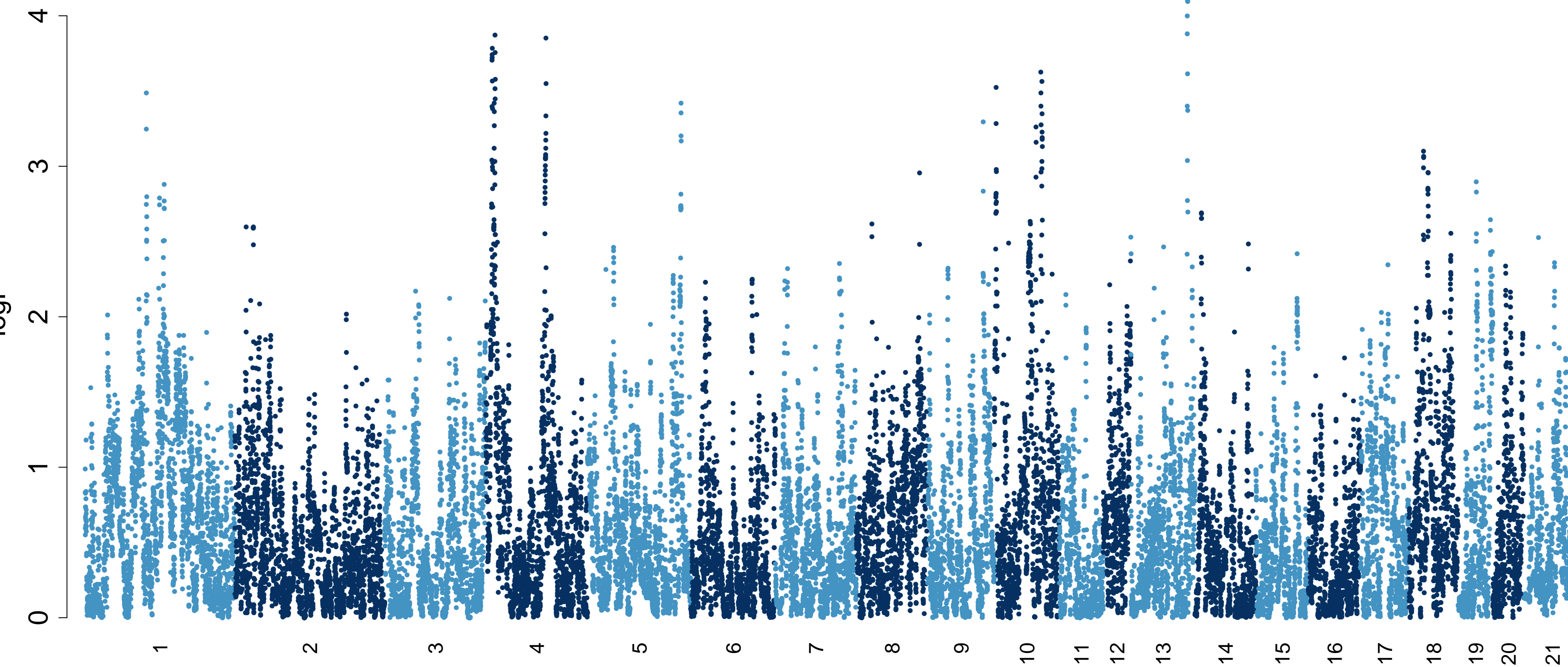
FACS_pctDN
