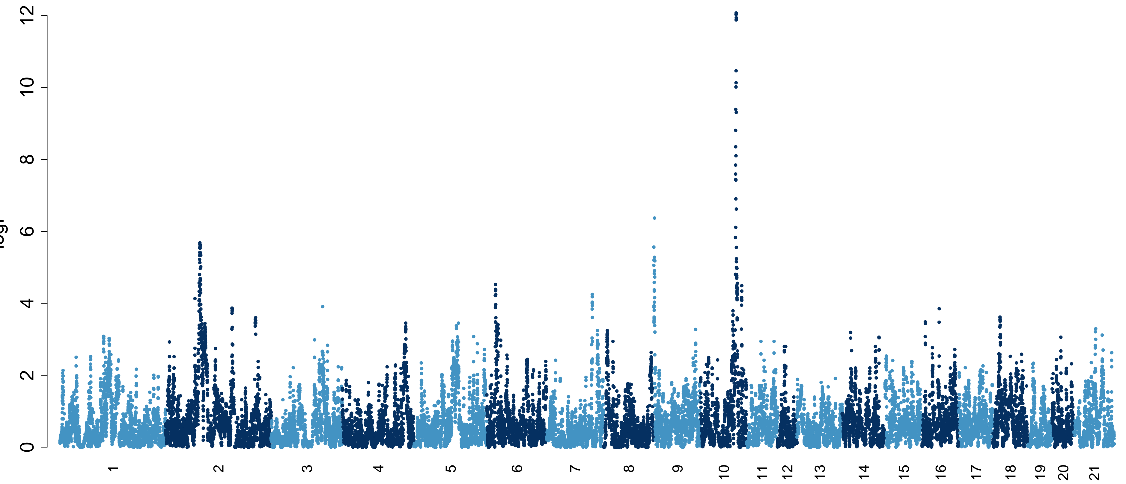
FACS_pctDP imputed
