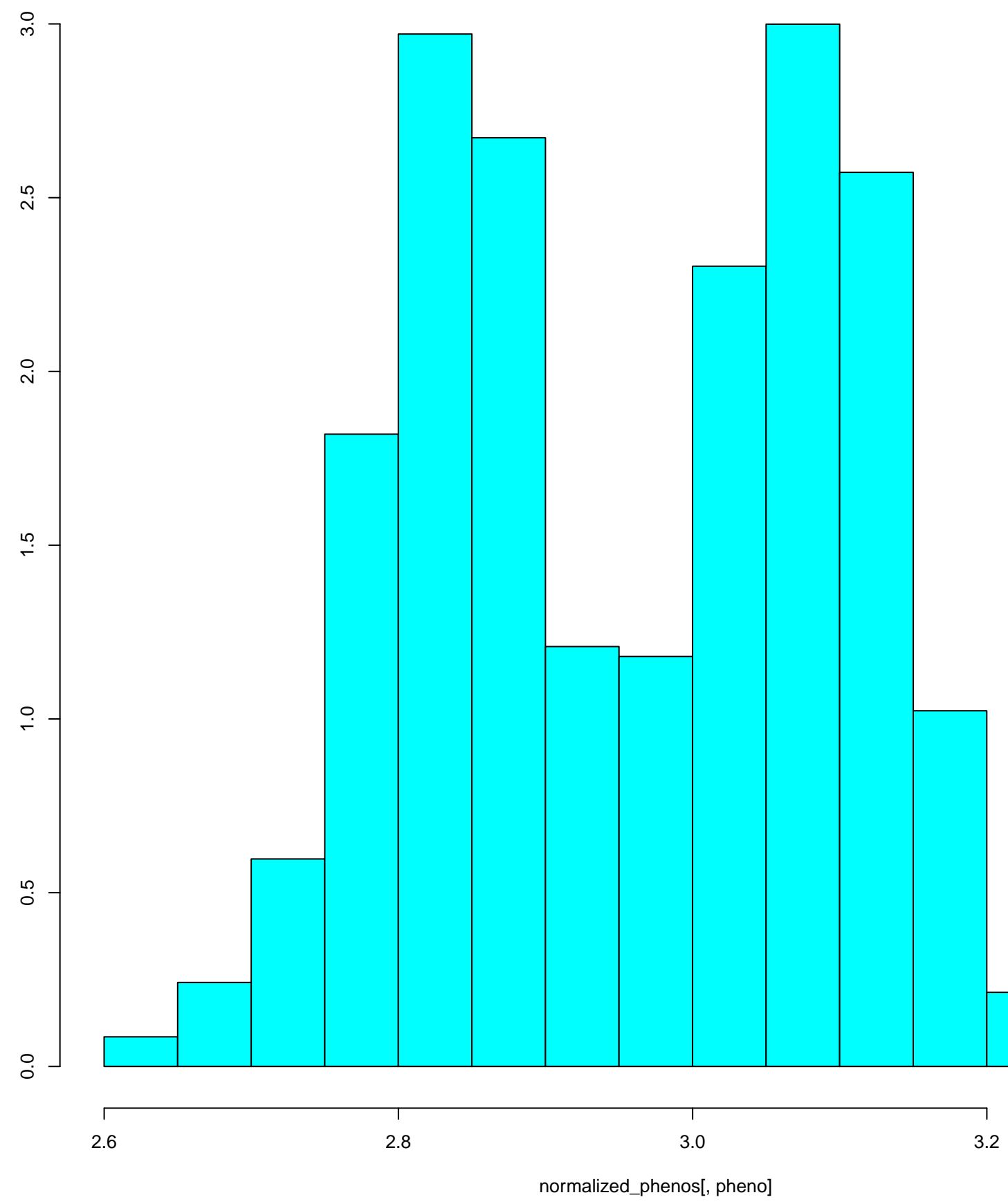
Normalized imputed pheno
