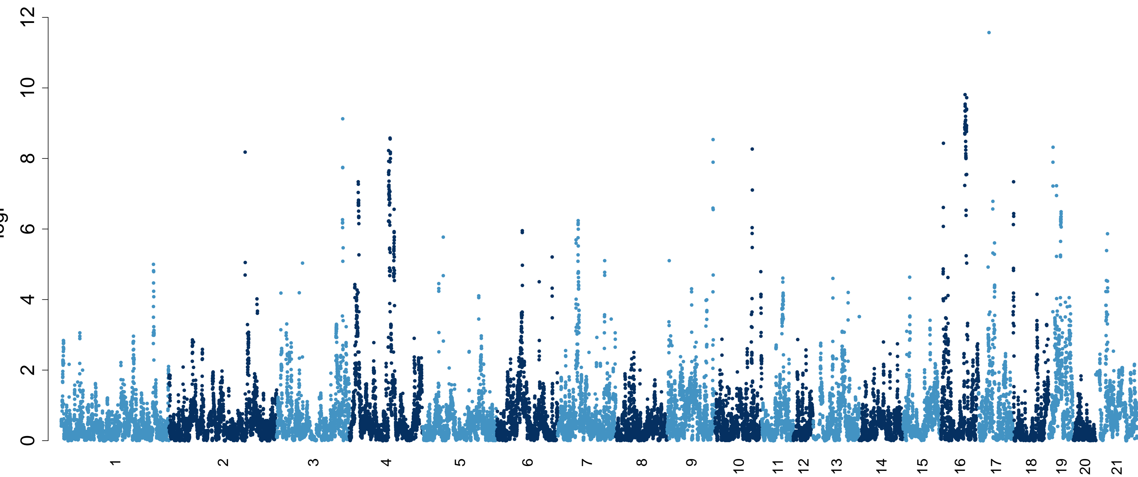
Hematology_MCHC imputed
