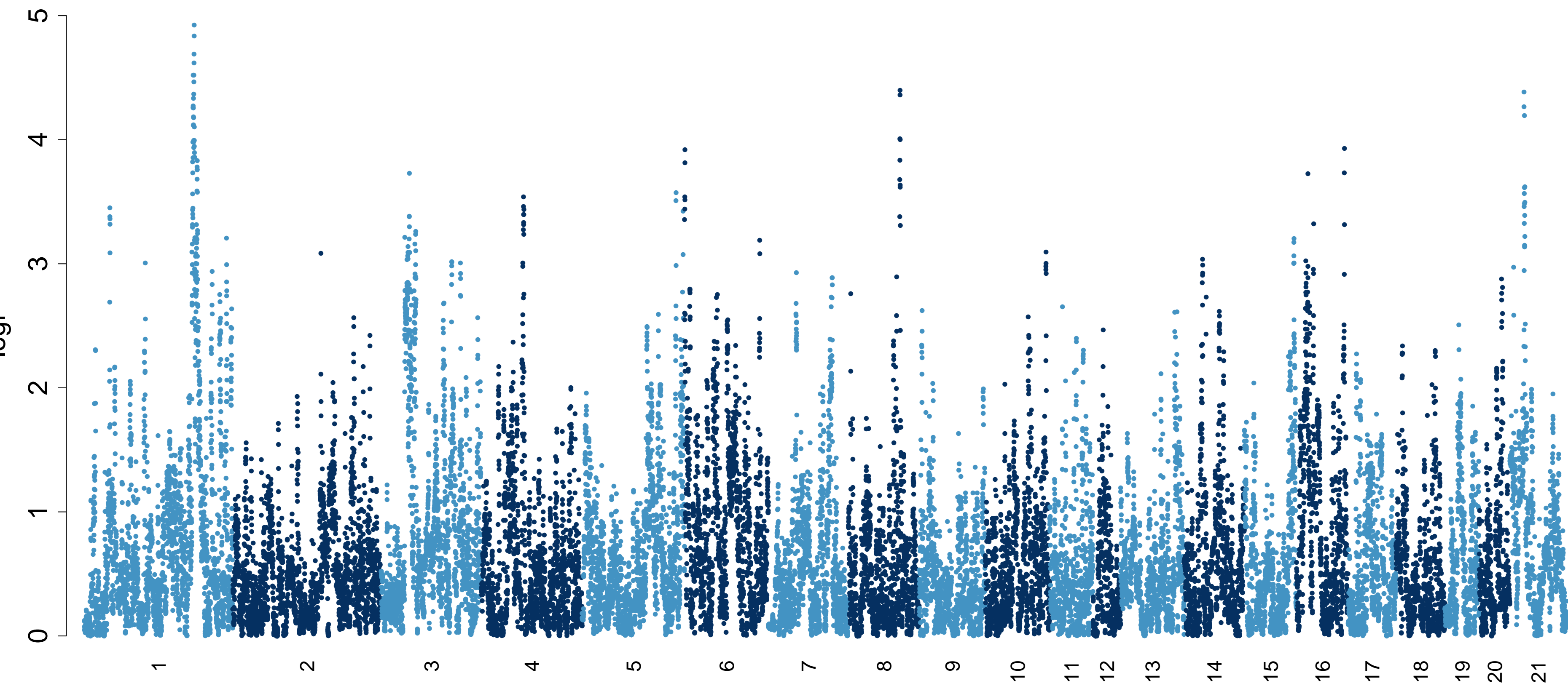
Shuttlebox_InterTrialCross1_20
