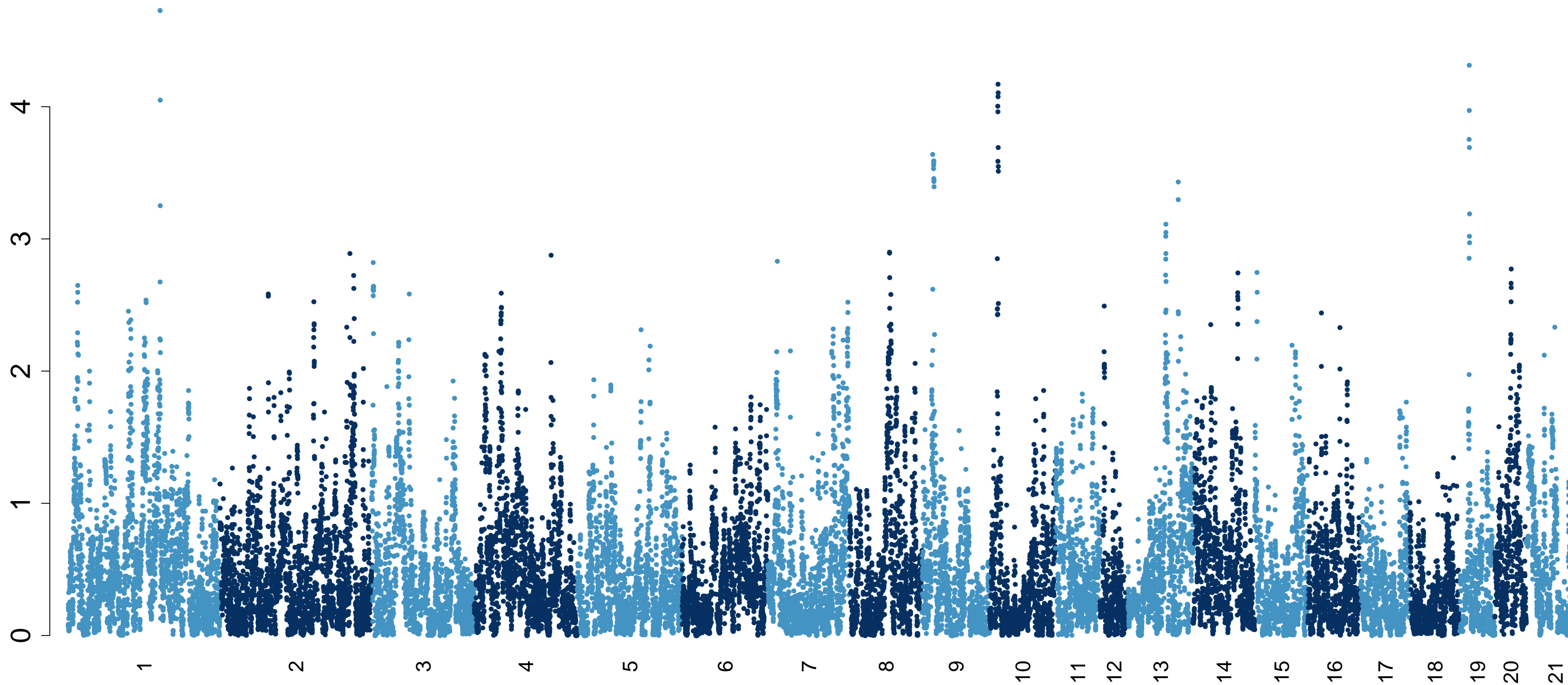
gls_design_Activity_Rearing15_20_bc_additive.txt
