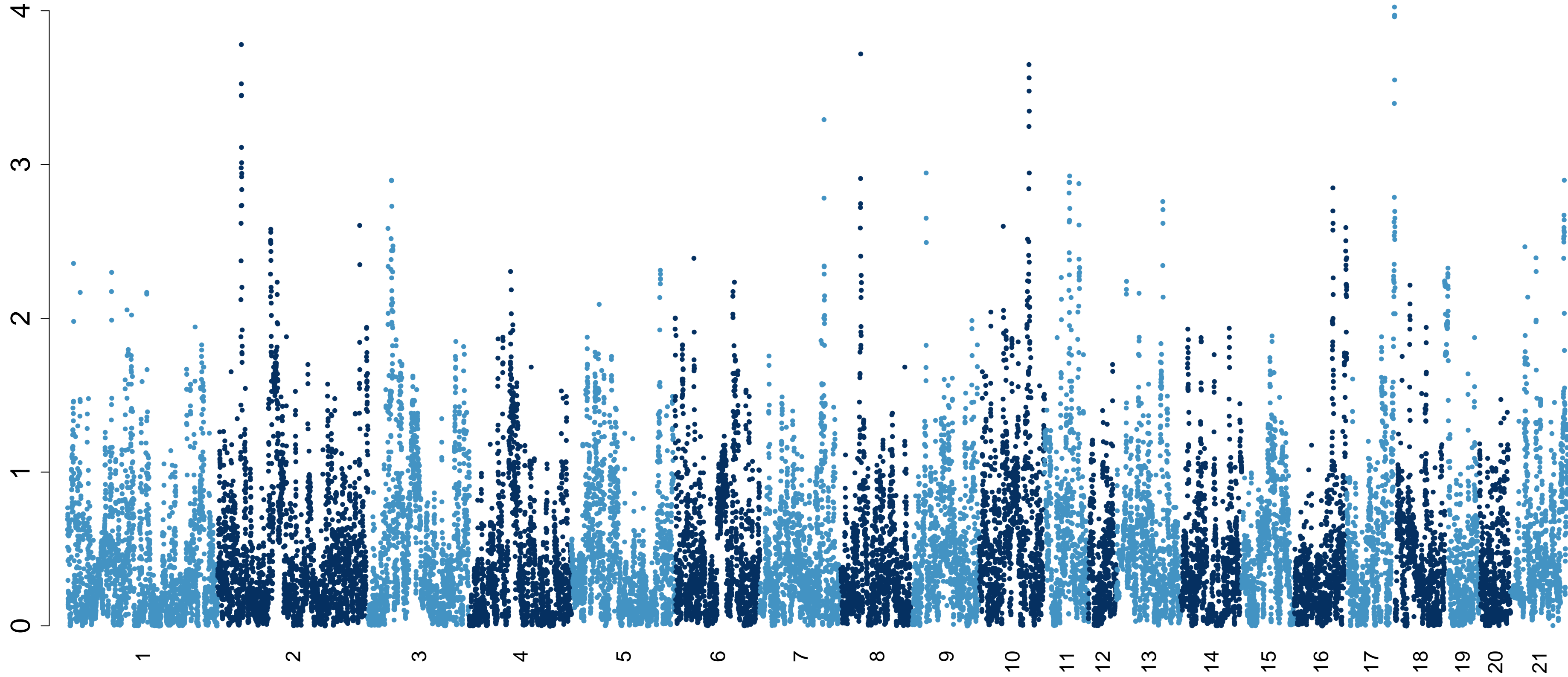
gls_design_Activity_Distance5_10_bc_additive.txt
