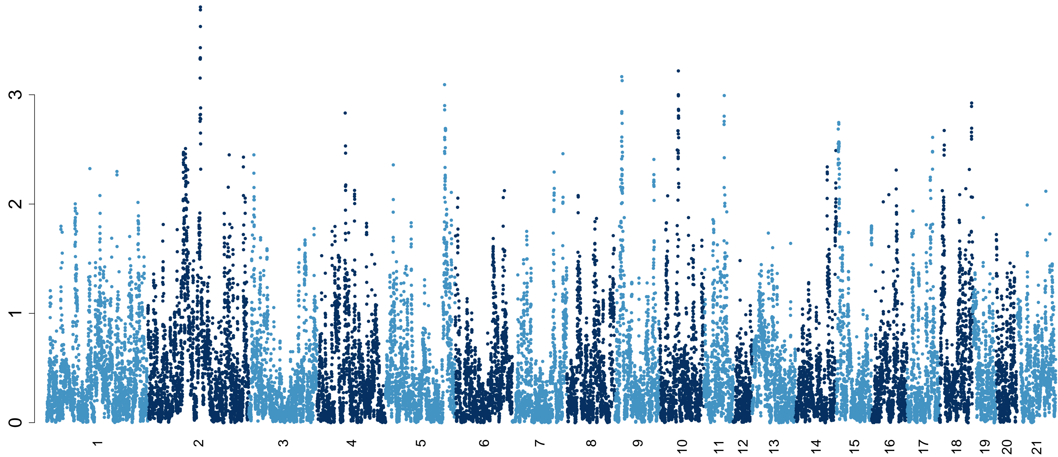
gls_design_Activity_Distance25_30_bc_additive.txt
