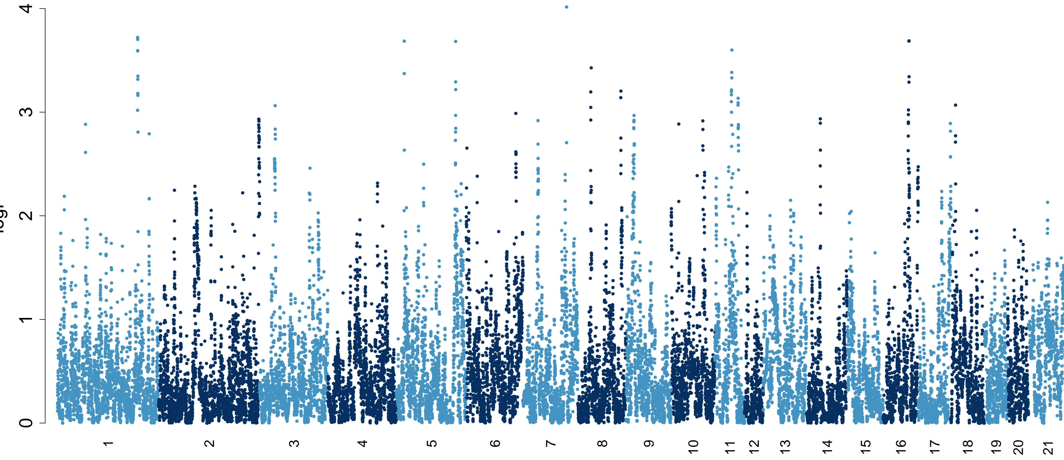
gls_design_Activity_Distance0_30_bc_additive.txt
