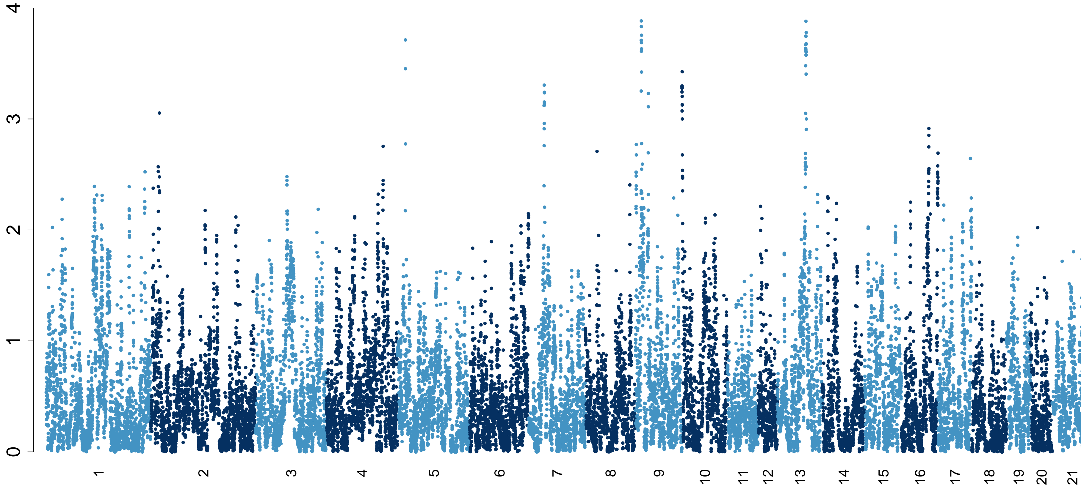
gls_design_Activity_Distance5_bc_additive.txt
