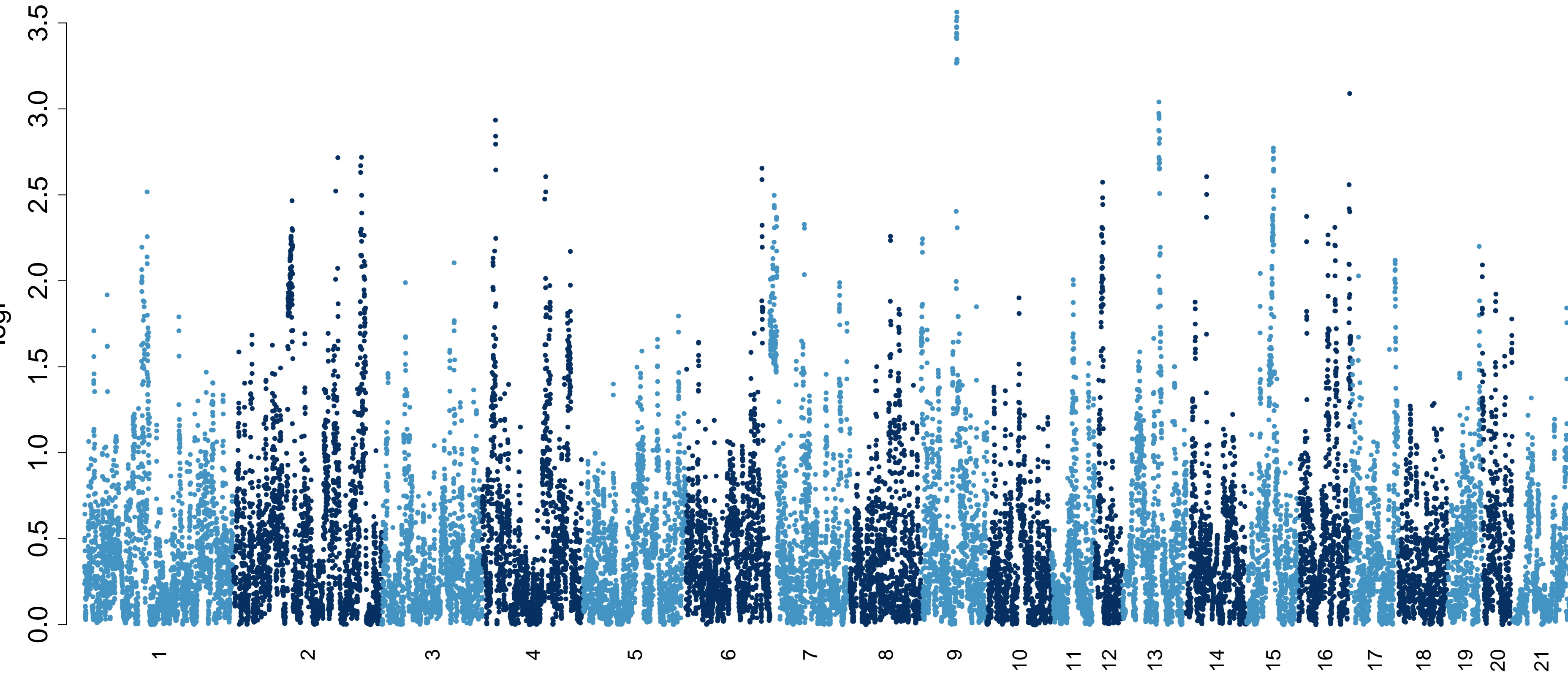
gls_design_Activity_Rearing20_25_bc_additive.txt
