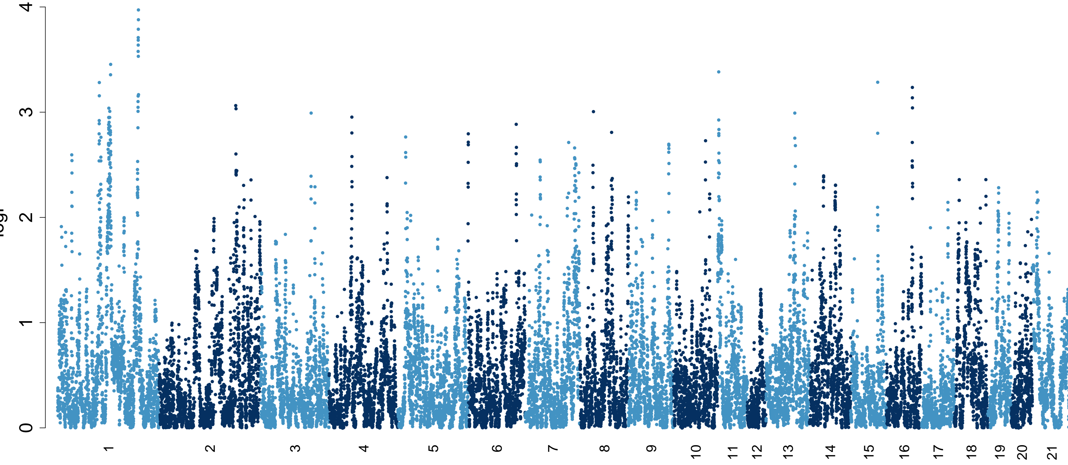
gls_design_Activity_Distance15_20_bc_additive.txt
