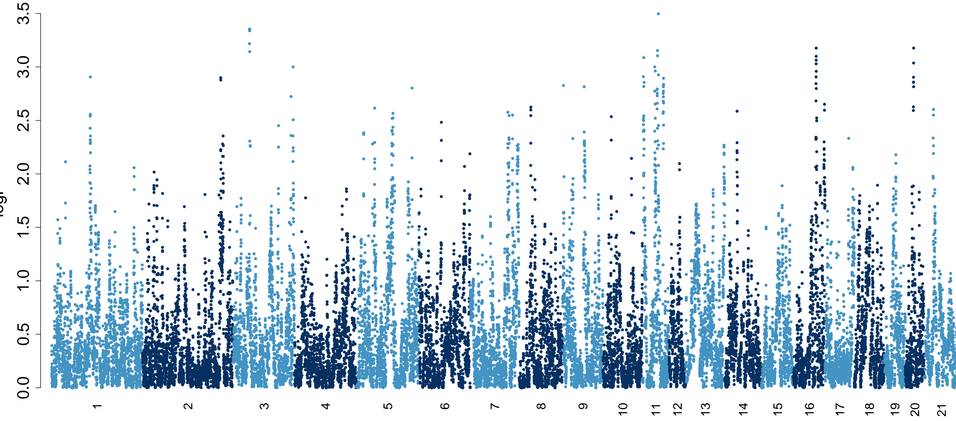
gls_design_Activity_Distance20_25_bc_additive.txt
