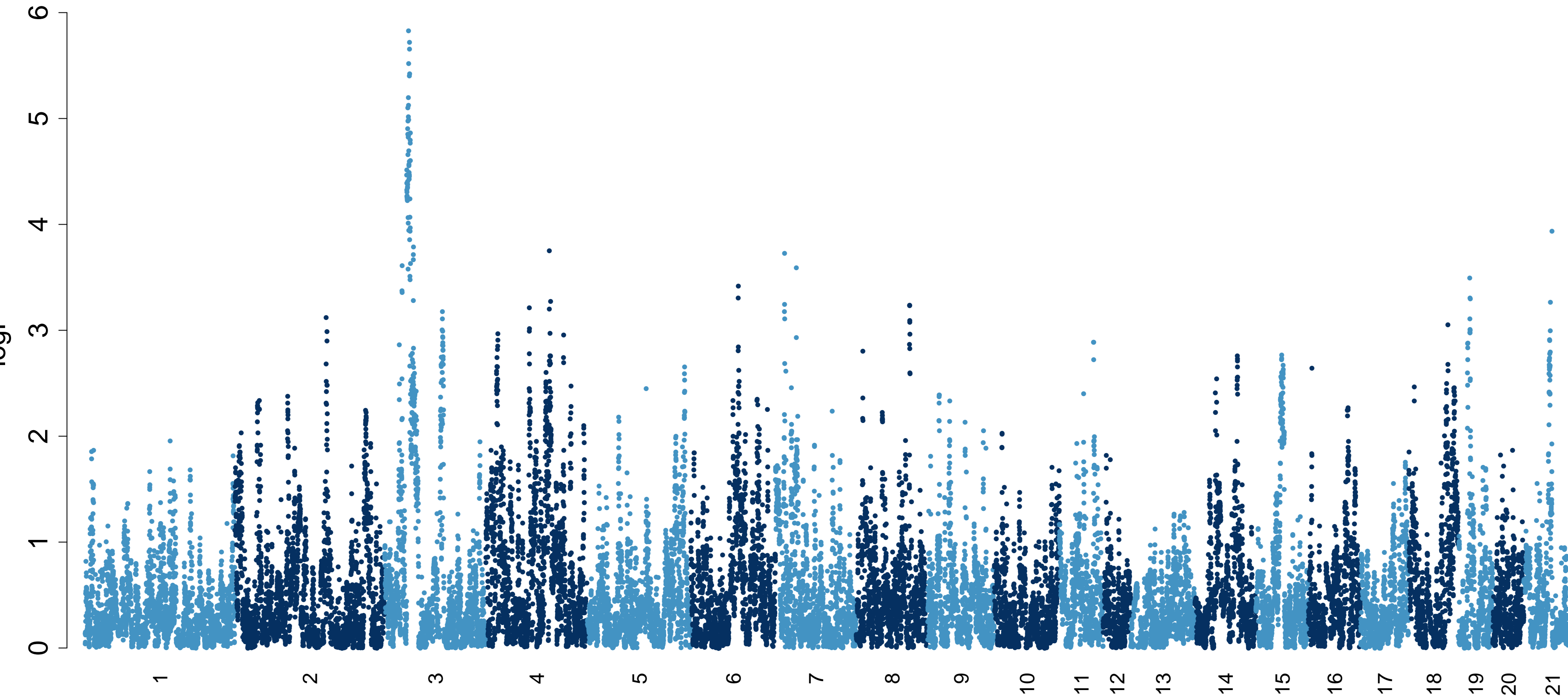
gls_design_Activity_Rearing10_15_bc_additive.txt
