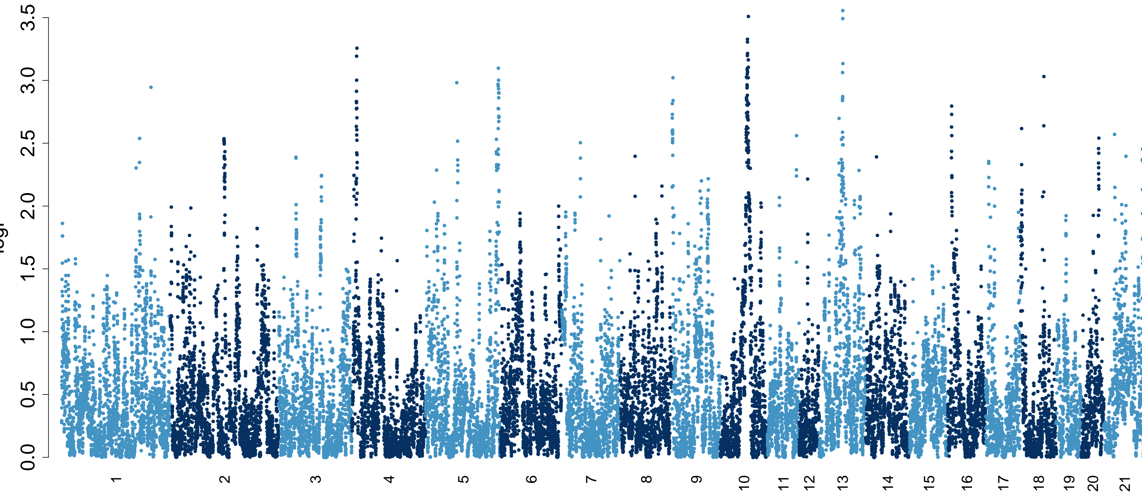
gls_design_FACS_pctCD45RClowCD8_additive.txt
