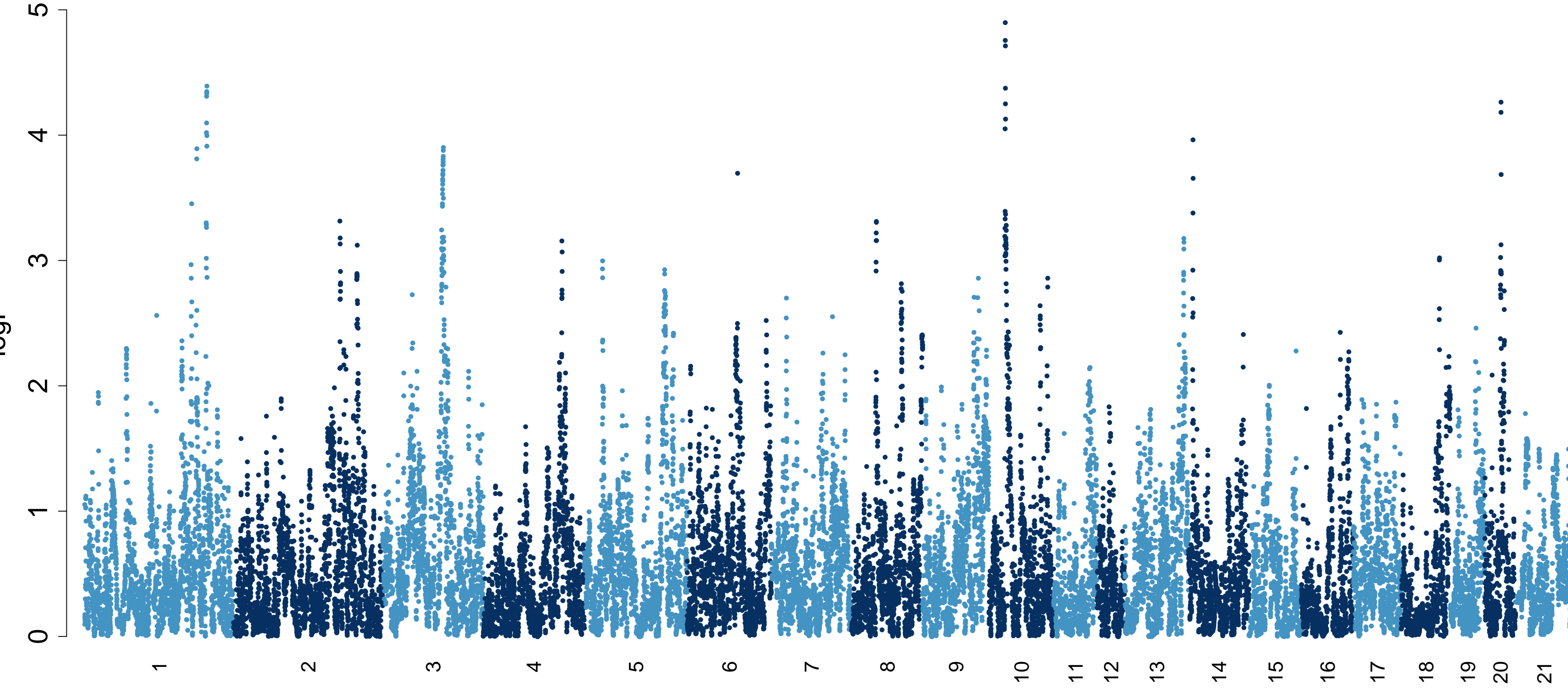
gls_design_FACS_Abs_gran_additive.txt
