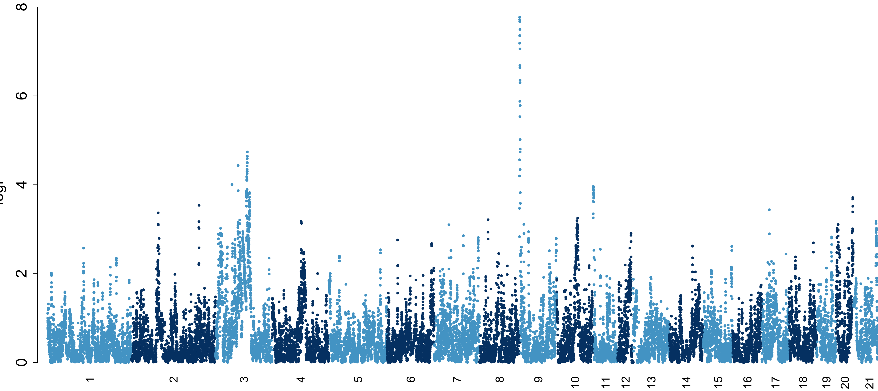
gls_design_FACS_WBCB_Abs_additive.txt
