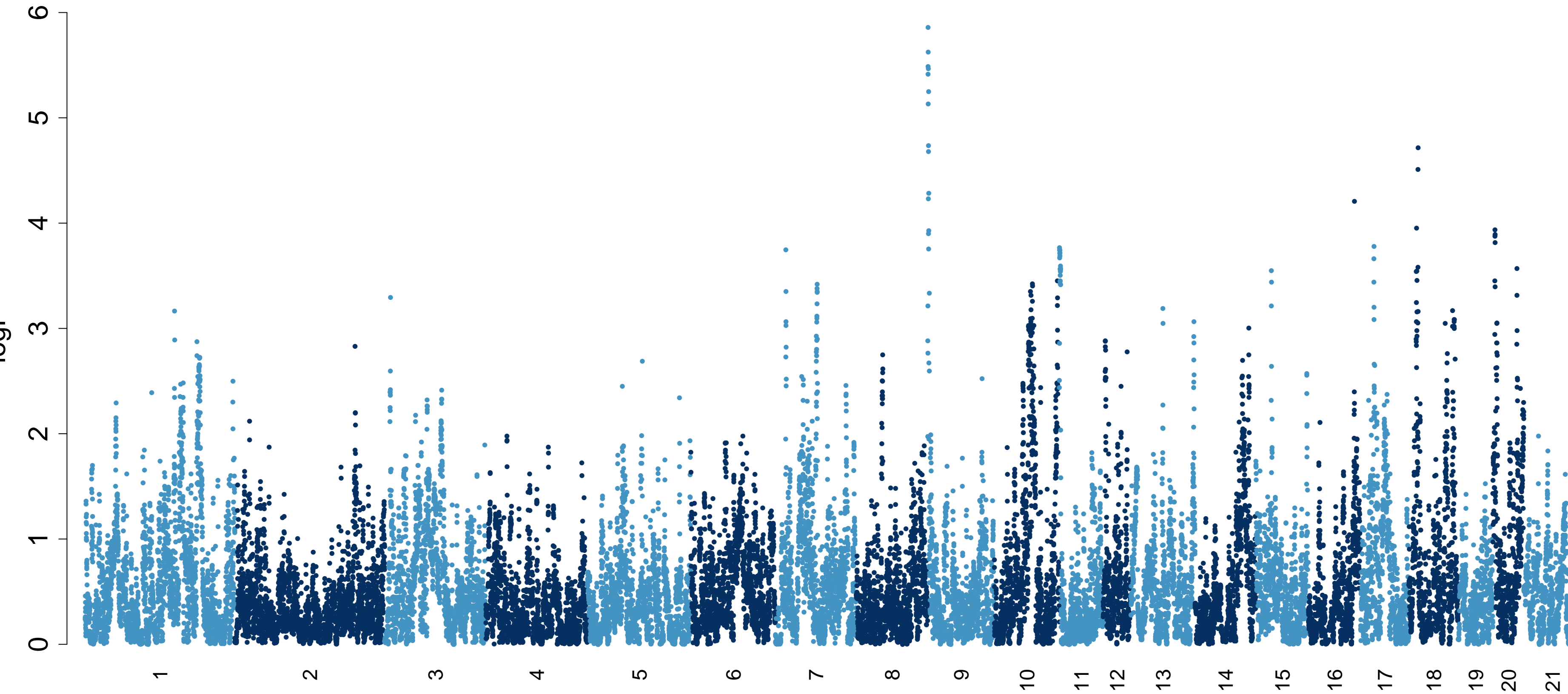
gls_design_FACS_Tcells_Abs_additive.txt
