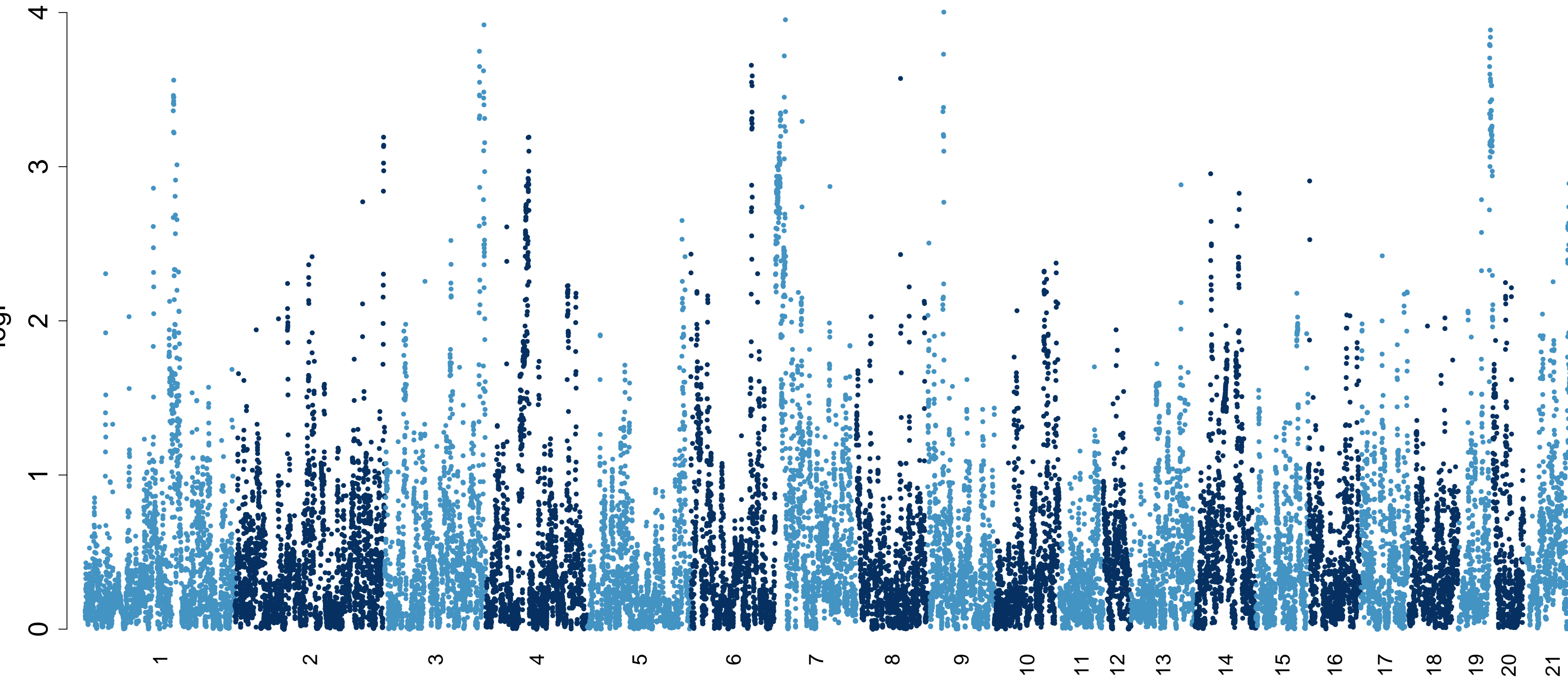
gls_design_FACS_CD25highCD8_additive.txt
