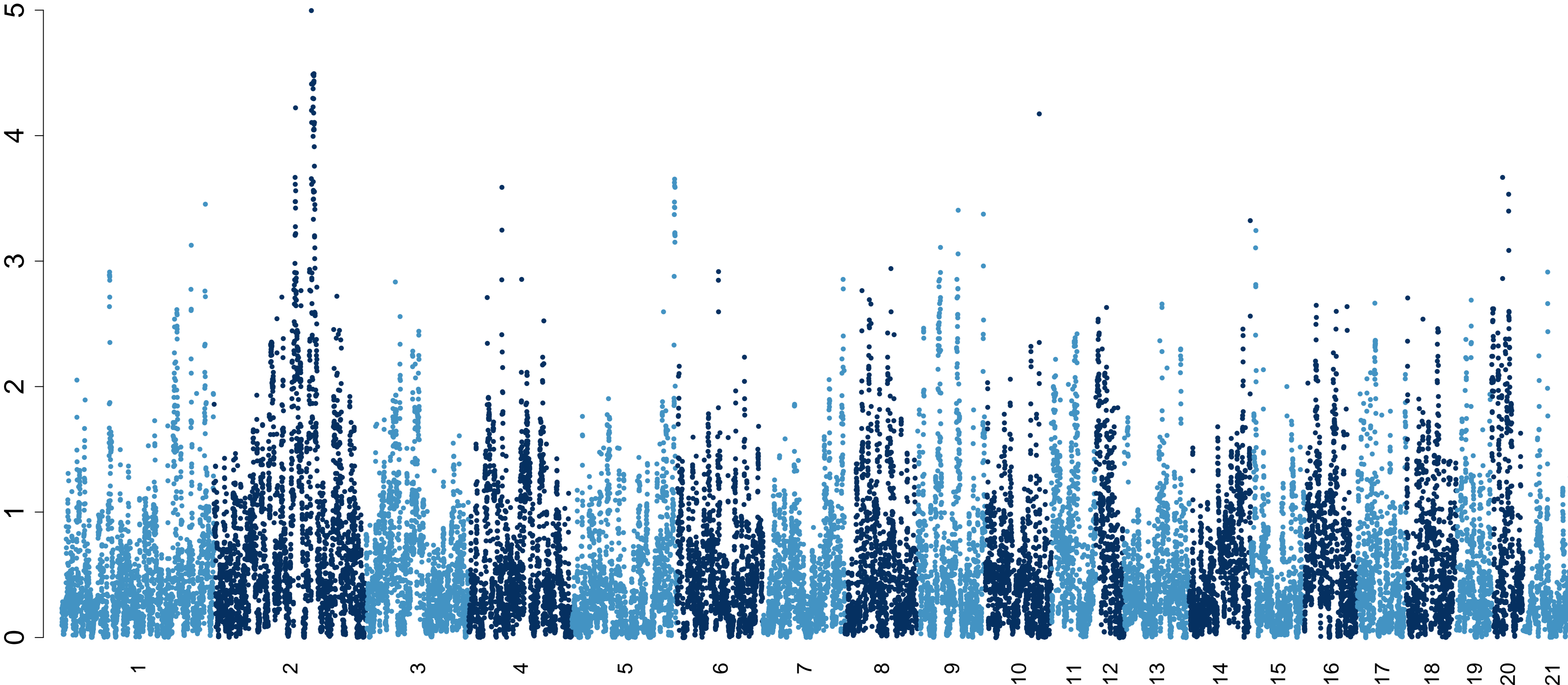
gls_design_General_BW_at_activity_test_bc_additive.txt
