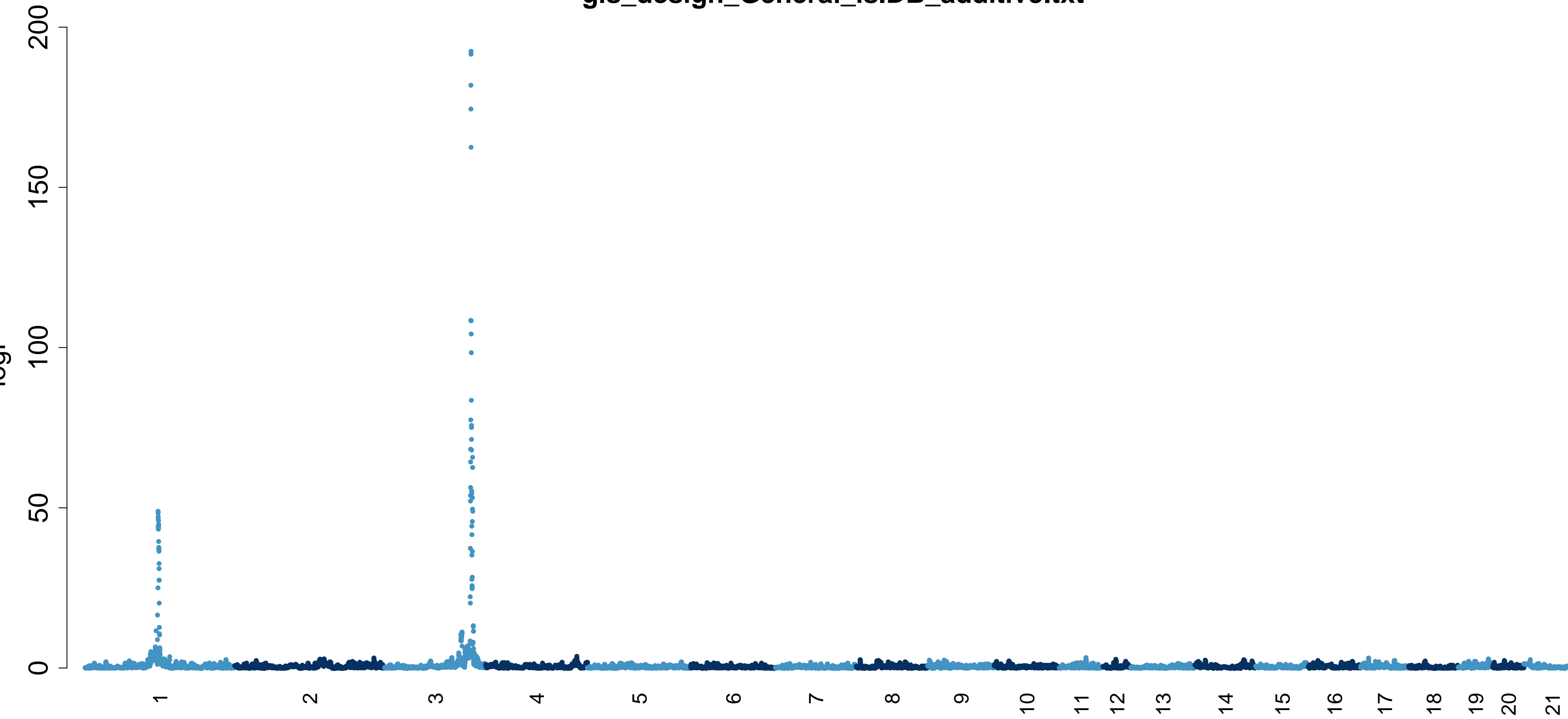
gls_design_General_is.DB_additive.txt
