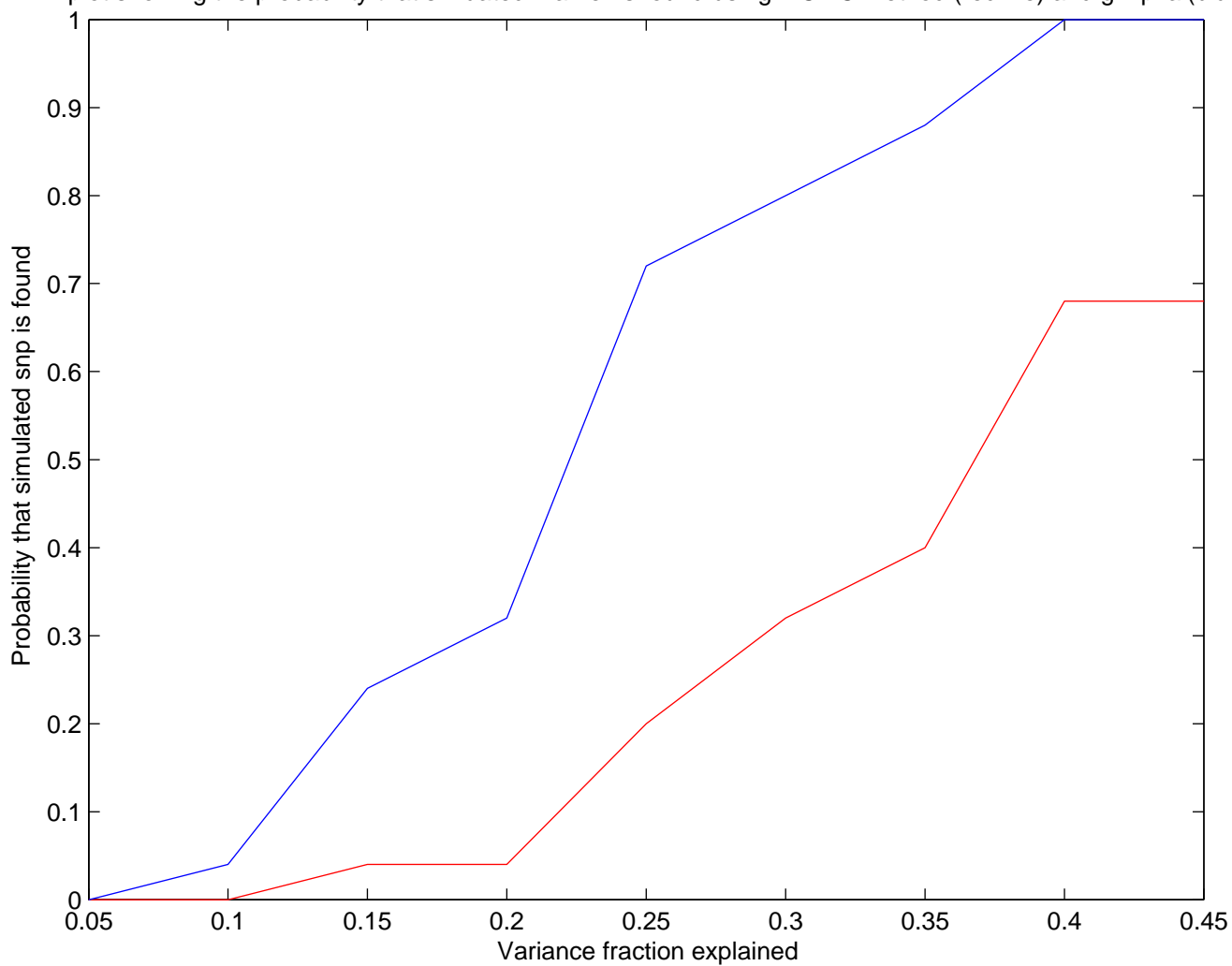
A plot showing the probability that simulated marker is found using MCMC method (redline) and glmpval(blue)
