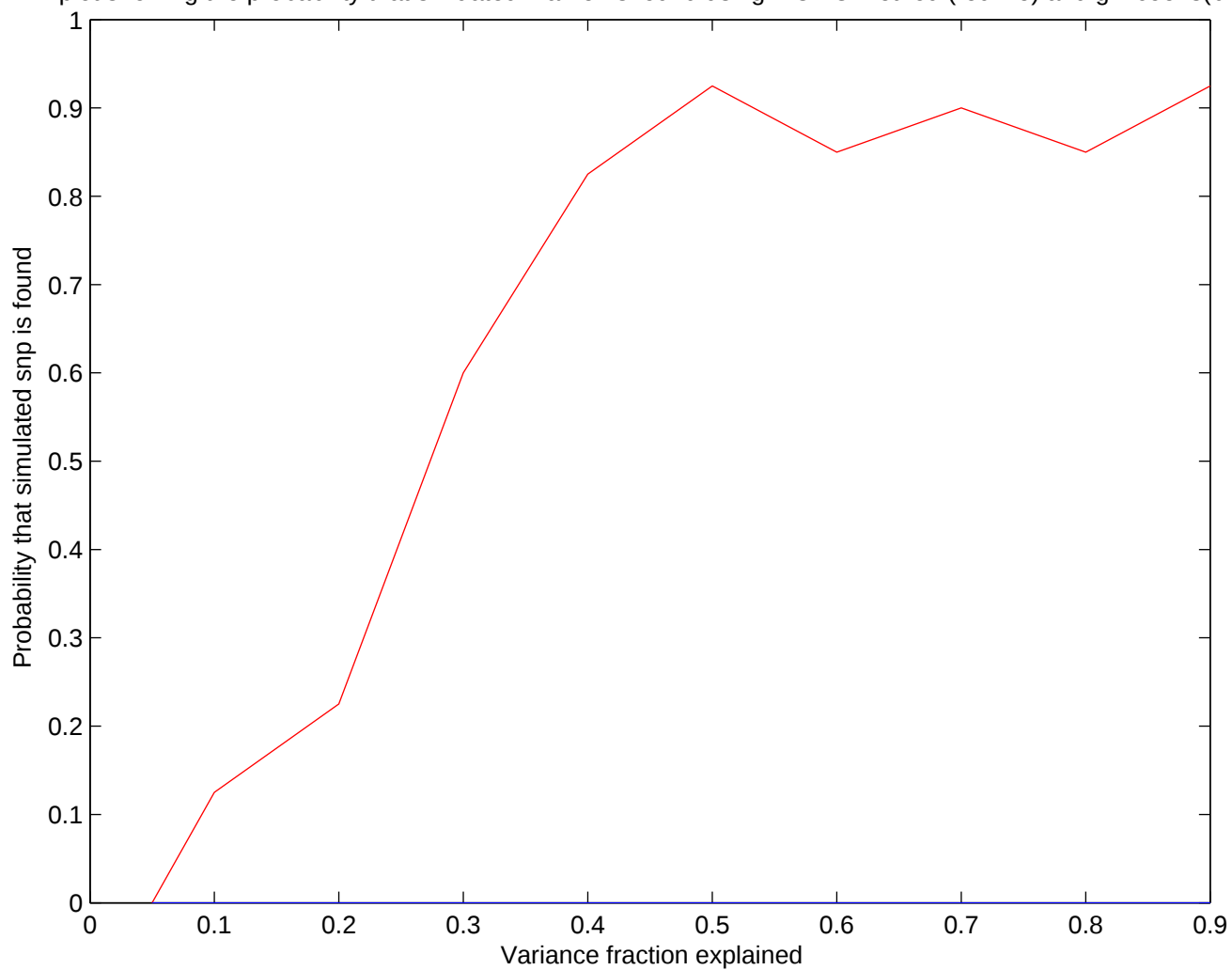
A plot showing the probability that simulated marker is found using MCMC method (redline) and glmcoeffs(blue)
