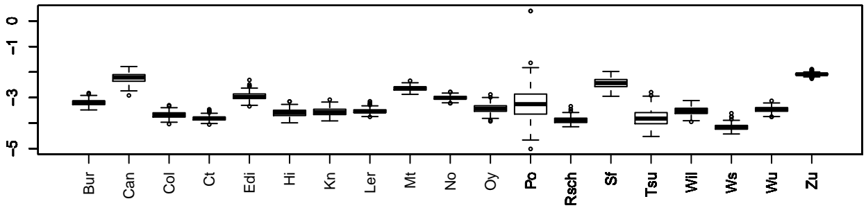
basal.given.days.to.bolt MN1_444820 chr3 6192392
