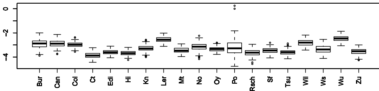
basal.given.days.to.bolt MN1_29716 chr1 17682800
