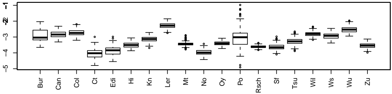
basal.given.days.to.bolt MN1_395107 chr1 23820733
