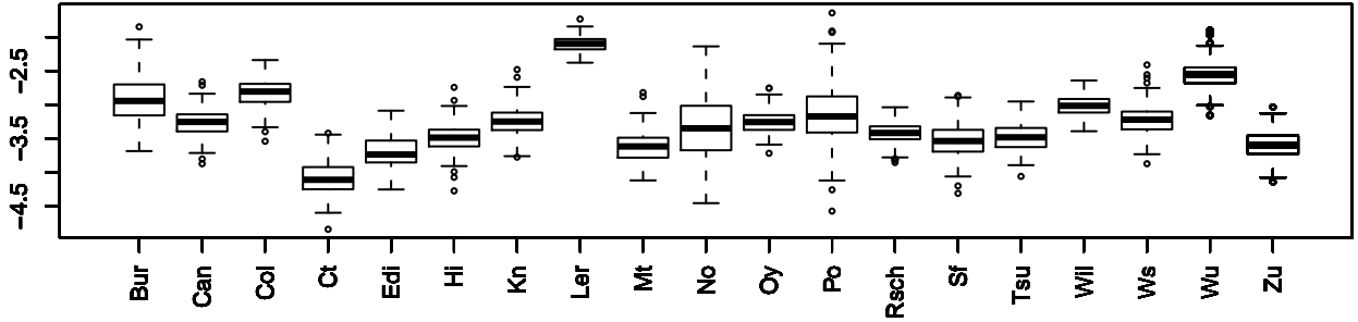
basal.given.days.to.bolt MASC03771 chr1 21140728
