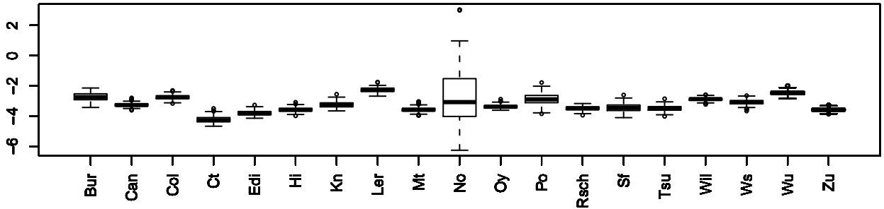
basal.given.days.to.bolt MN1_340810 chr1 21908604
