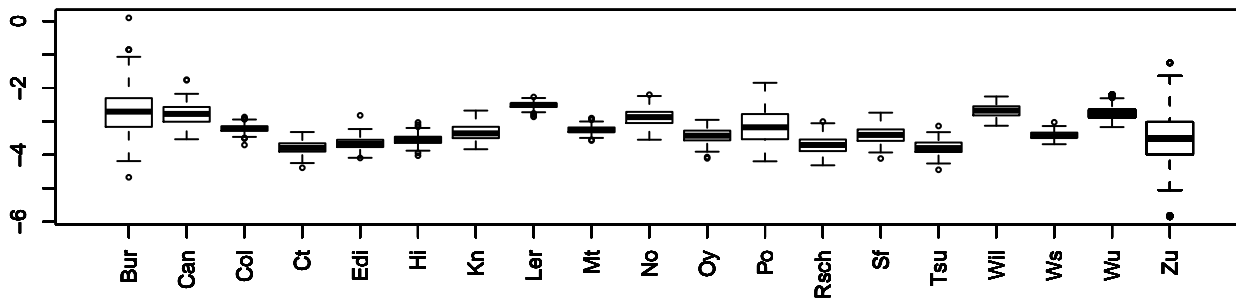
basal.given.days.to.bolt MN1_29291 chr1 16130993
