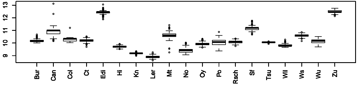
bolt.to.flower MN1_197787 chr5 4318002
