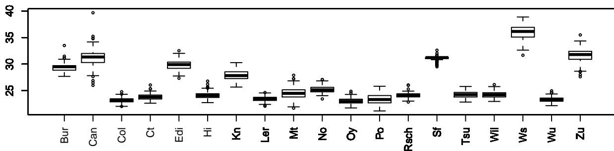
days.to.bolt MN1_29716 chr4 270863
