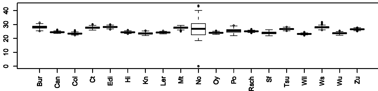
days.to.bolt MN1_29291 chr1 21908604
