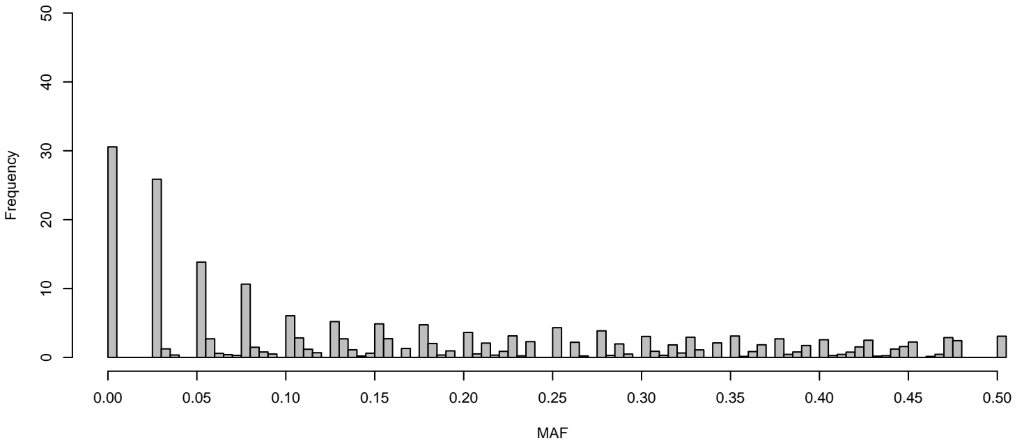
Probability of MAFs on Chr 18 (grey = all, blue = known, red = new)
