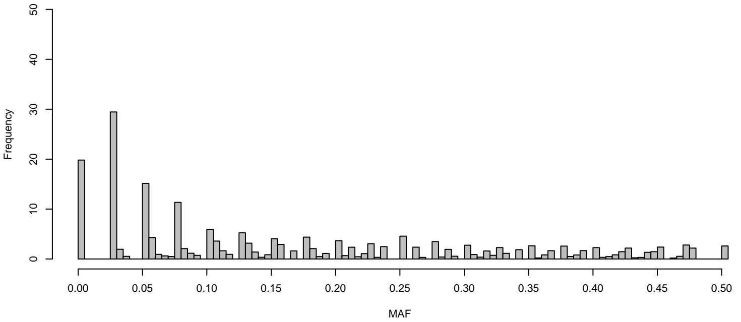
Probability of MAFs on Chr 12 (grey = all, blue = known, red = new)
