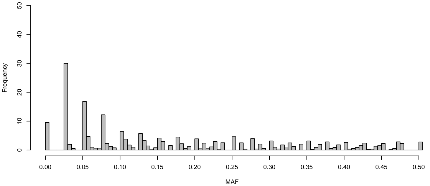
Probability of MAFs on Chr 5 (grey = all, blue = known, red = new)
