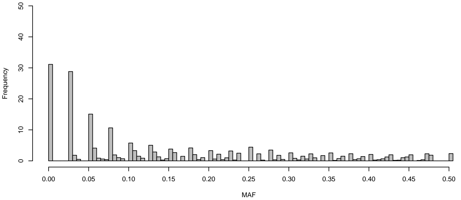
Probability of MAFs on Chr 8 (grey = all, blue = known, red = new)
