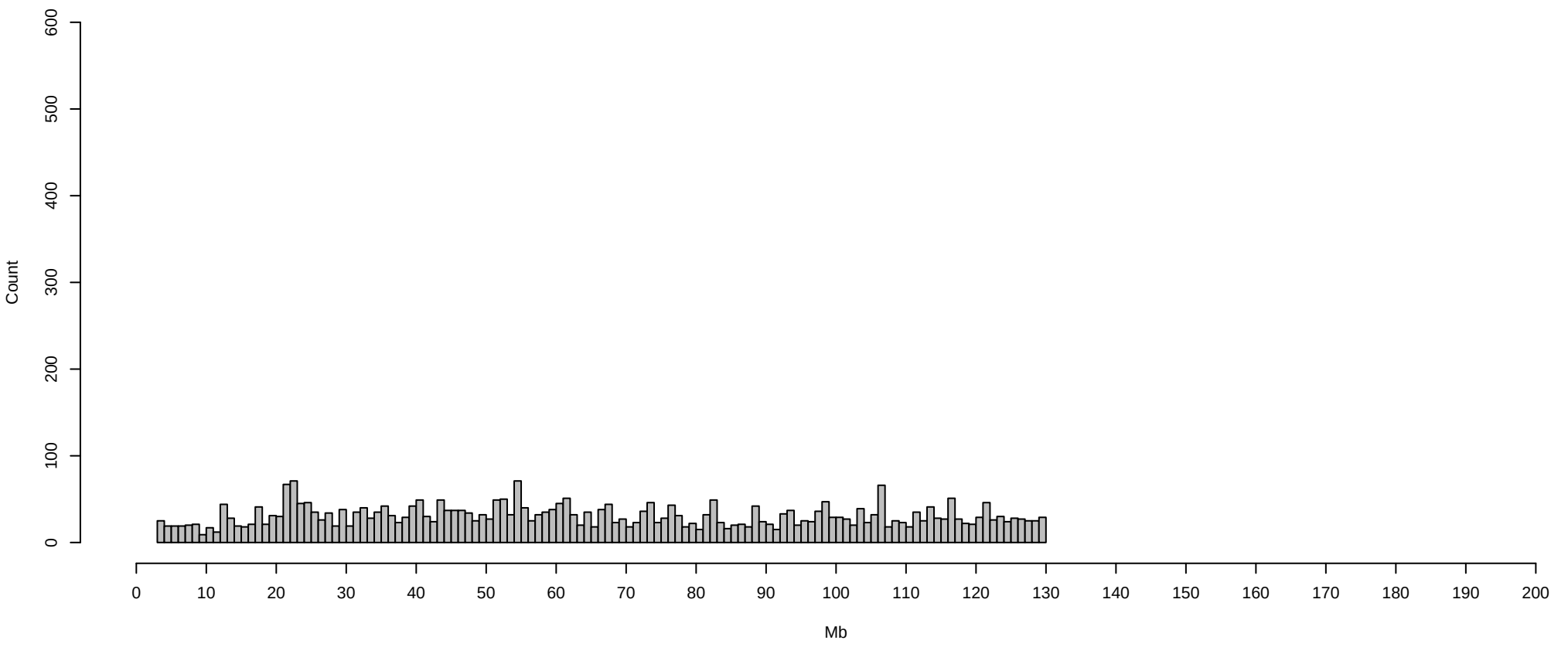
Chromosome 10 counts of snps with multiple ALTs
