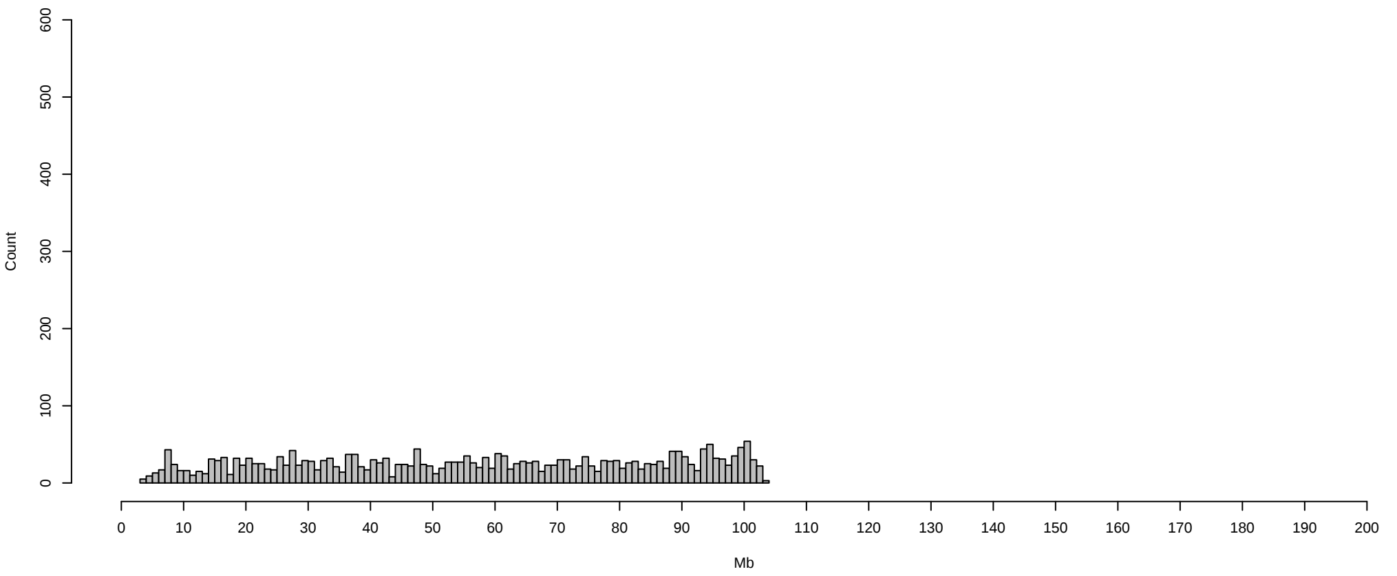
Chromosome 15 counts of snps with multiple ALTs
