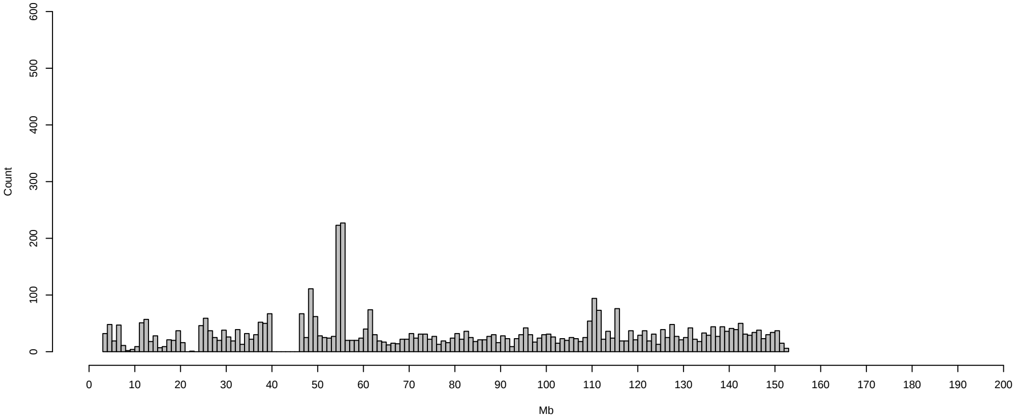
Chromosome 7 counts of snps with multiple ALTs
