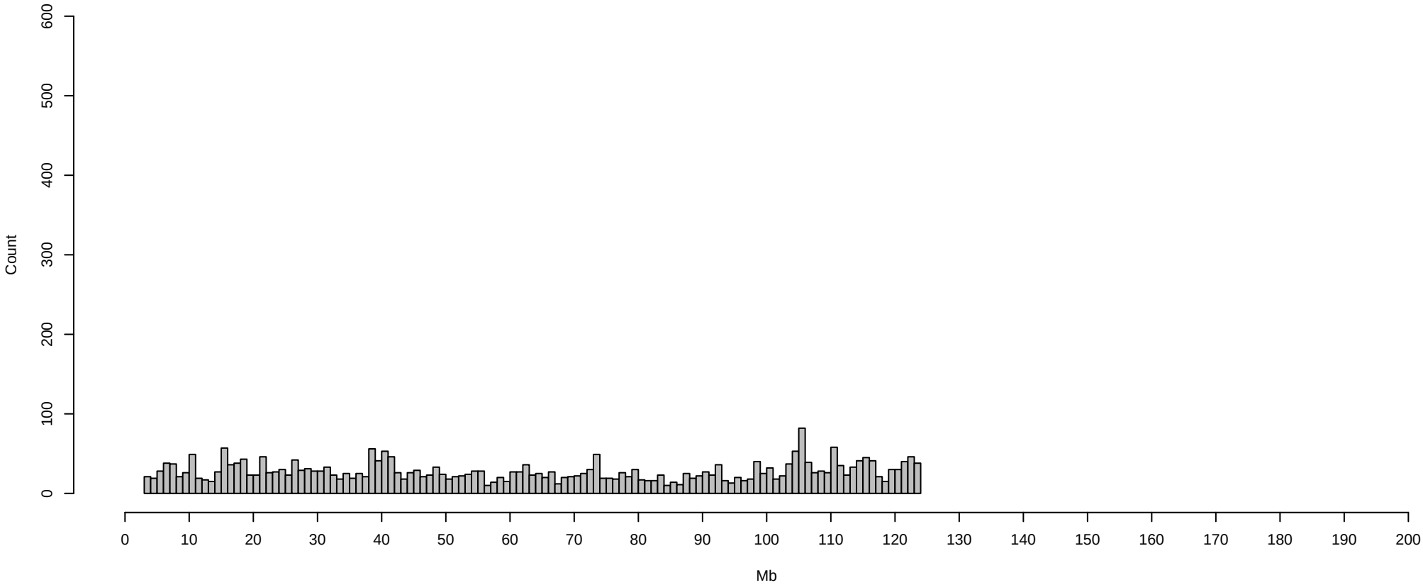
Chromosome 9 counts of snps with multiple ALTs
