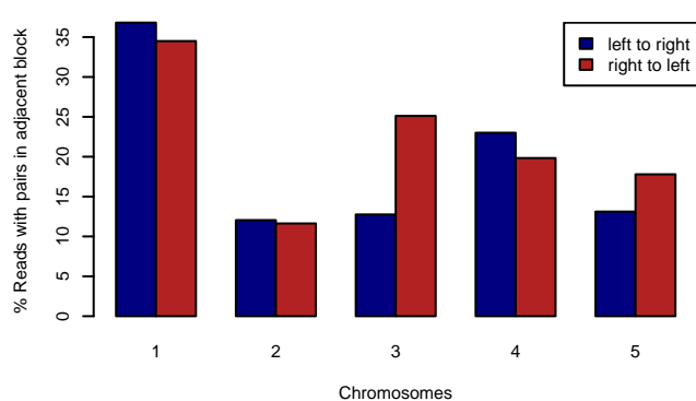
MAGIC.426 – RELIABLE.BPS
