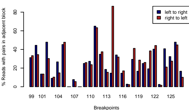
MAGIC.149 – RELIABLE.BPS
