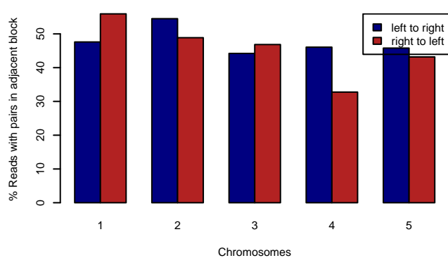
MAGIC.426 – CONTROLLERS
