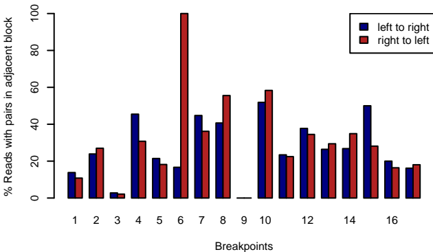
MAGIC.338 – RELIABLE.BPS
