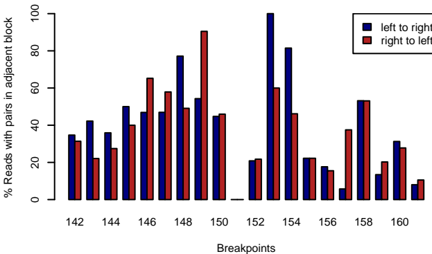
MAGIC.433 – RELIABLE.BPS
