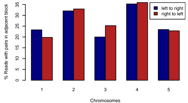
MAGIC.338 – RELIABLE.BPS
