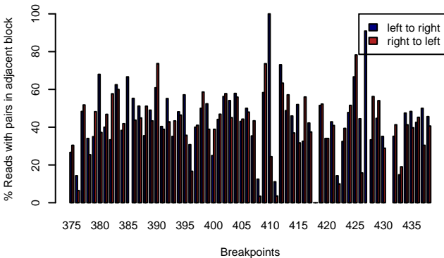
MAGIC.446 – CONTROLLERS
