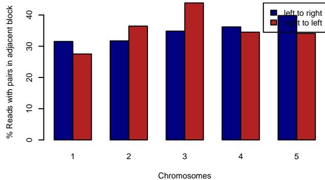
MAGIC.175 – RELIABLE.BPS
