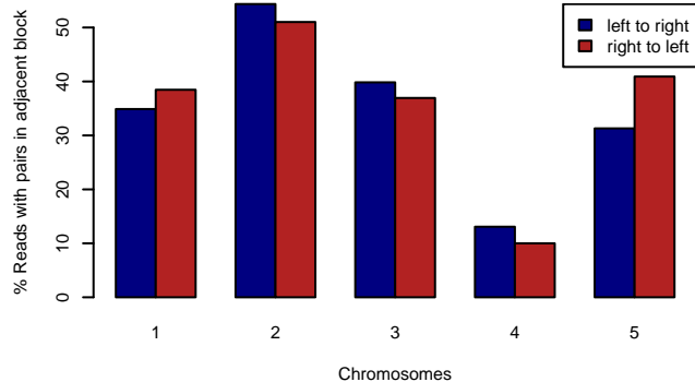
MAGIC.287 – RELIABLE.BPS
