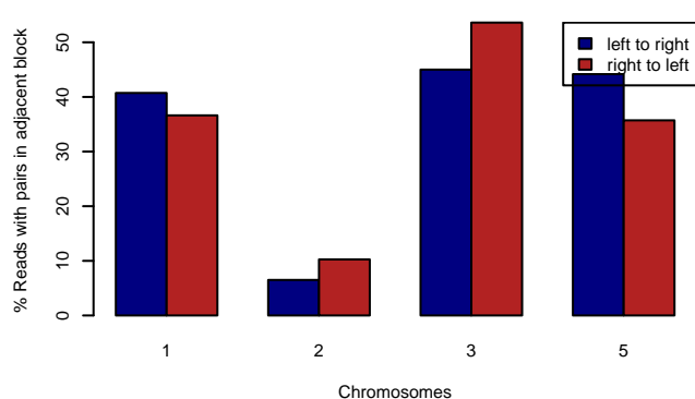
MAGIC.426 – DENSE.BPS
