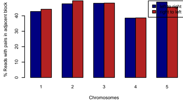
MAGIC.287 – DENSE.BPS
