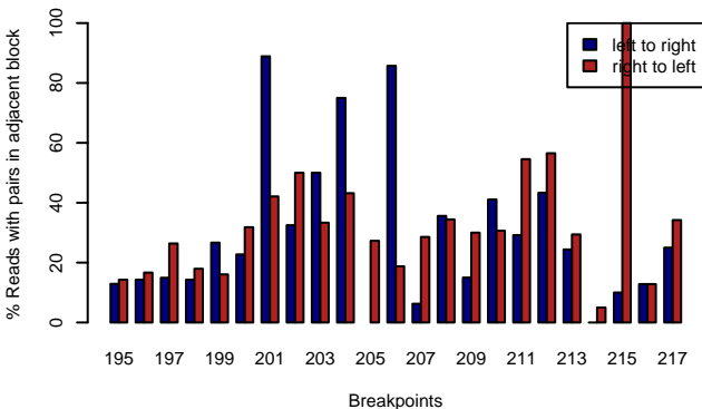
MAGIC.149 – DENSE.BPS
