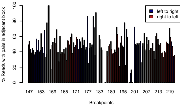
MAGIC.329 – CONTROLLERS
