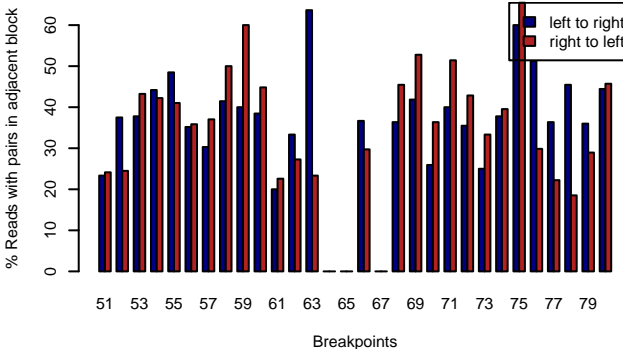
MAGIC.287 – RELIABLE.BPS
