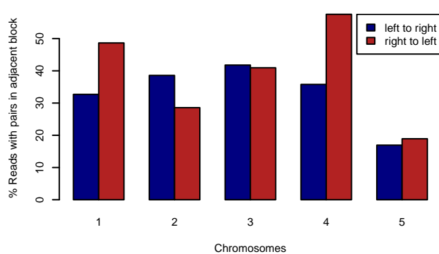
MAGIC.446 – RELIABLE.BPS
