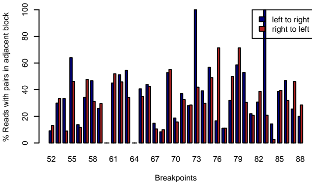
MAGIC.329 – RELIABLE.BPS
