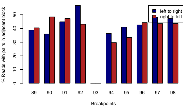
MAGIC.105 – RELIABLE.BPS
