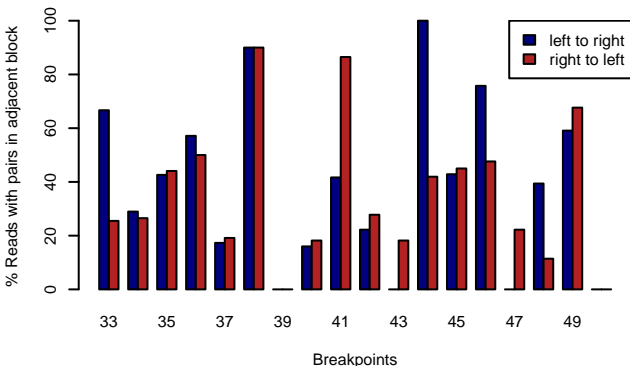
MAGIC.426 – DENSE.BPS
