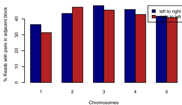
MAGIC.446 – CONTROLLERS
