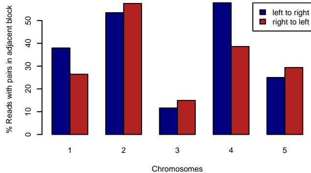
MAGIC.433 – RELIABLE.BPS
