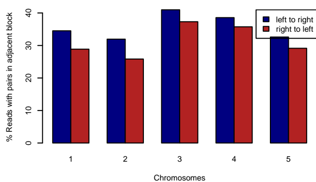
MAGIC.329 – RELIABLE.BPS
