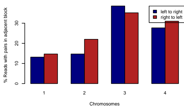
MAGIC.149 – DENSE.BPS
