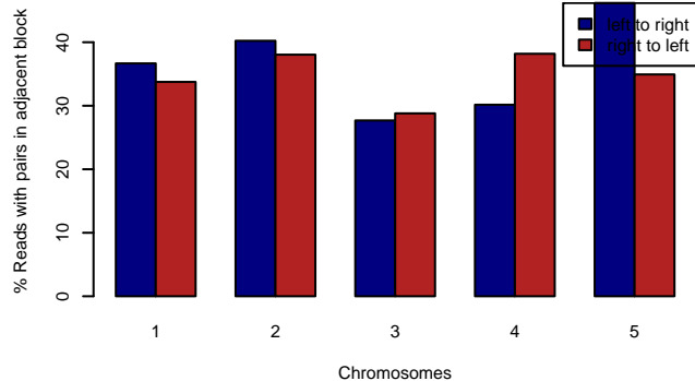
MAGIC.287 – RELIABLE.BPS
