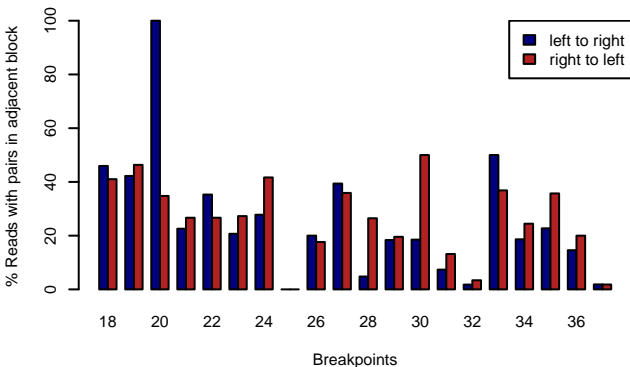
MAGIC.426 – RELIABLE.BPS
