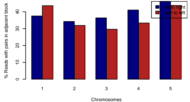
MAGIC.105 – RELIABLE.BPS
