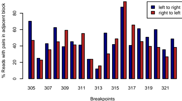
MAGIC.175 – RELIABLE.BPS
