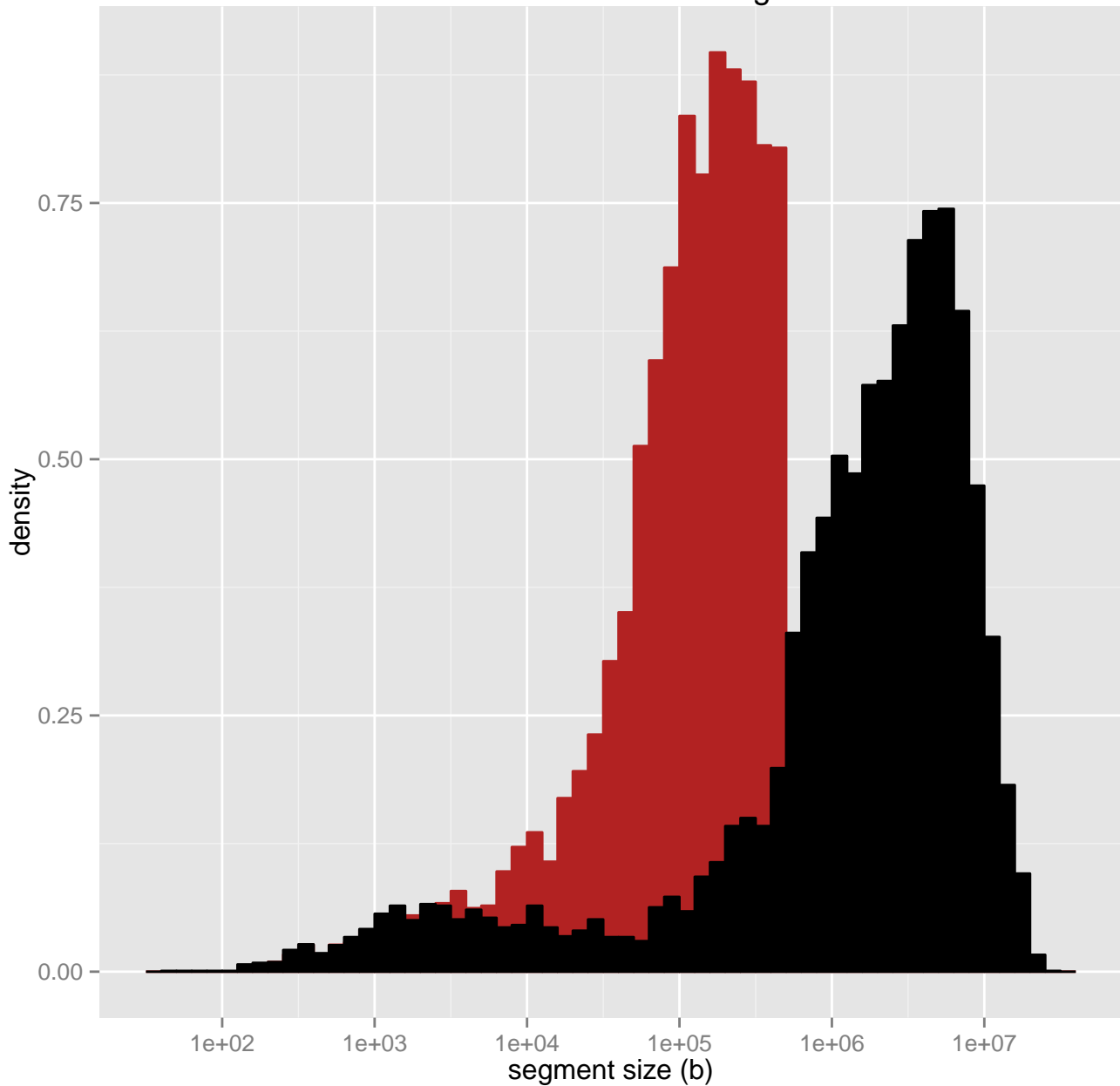
Distribution of unrecombined segment sizes
