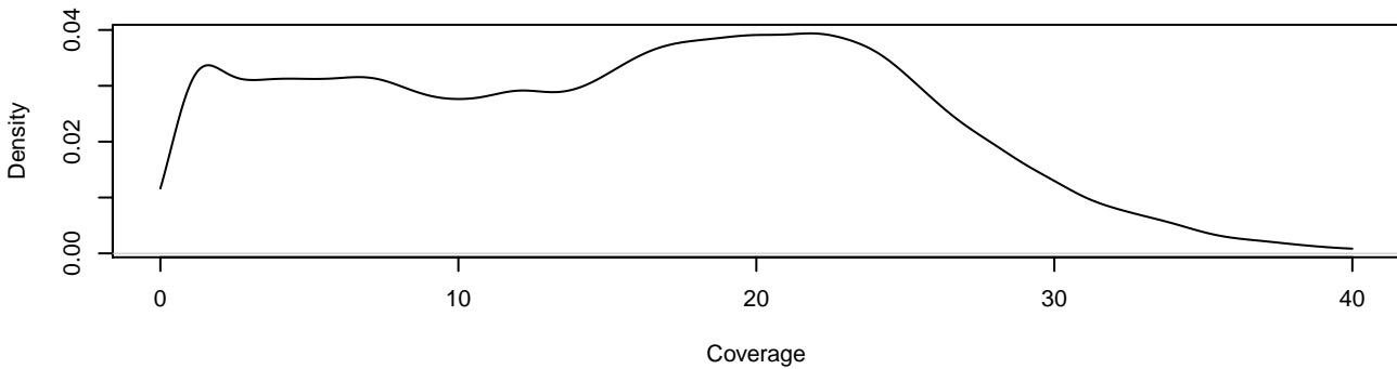
Coverage of very dense breakpoints (distance < 50kb) from = 0 to = 40
