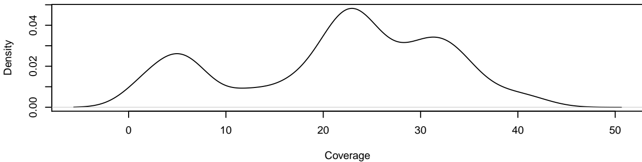
MAGIC.175 1 22855995 22856029
