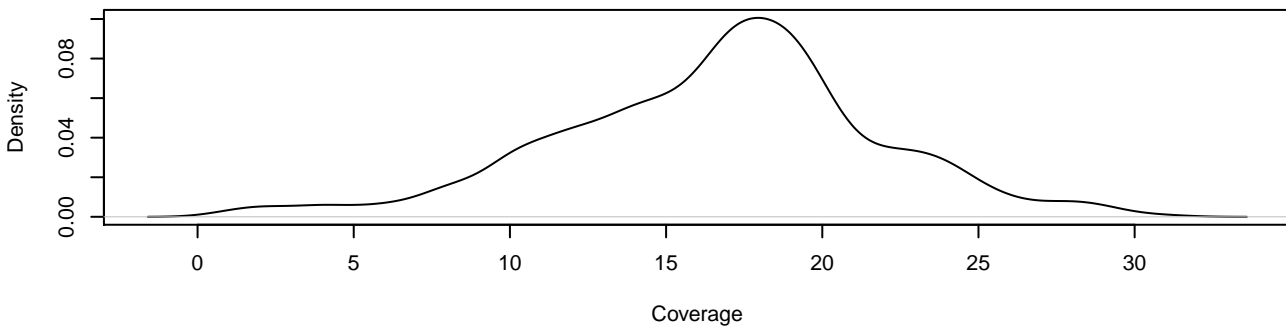
MAGIC.175 5 5675077 5675100
