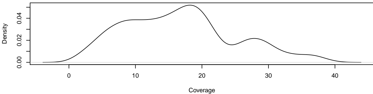
MAGIC.175 1 22842808 22842809
