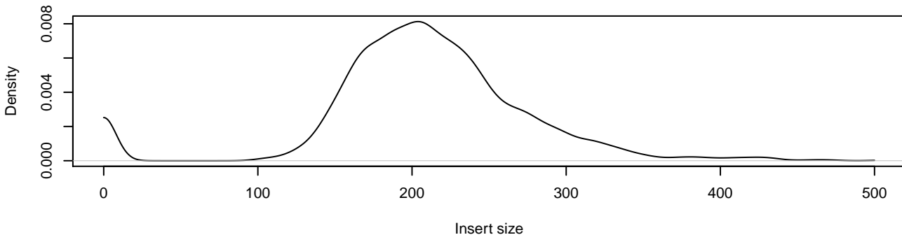
Insert size inside haplotype blocks (controllers)from = 0 to = 1000
