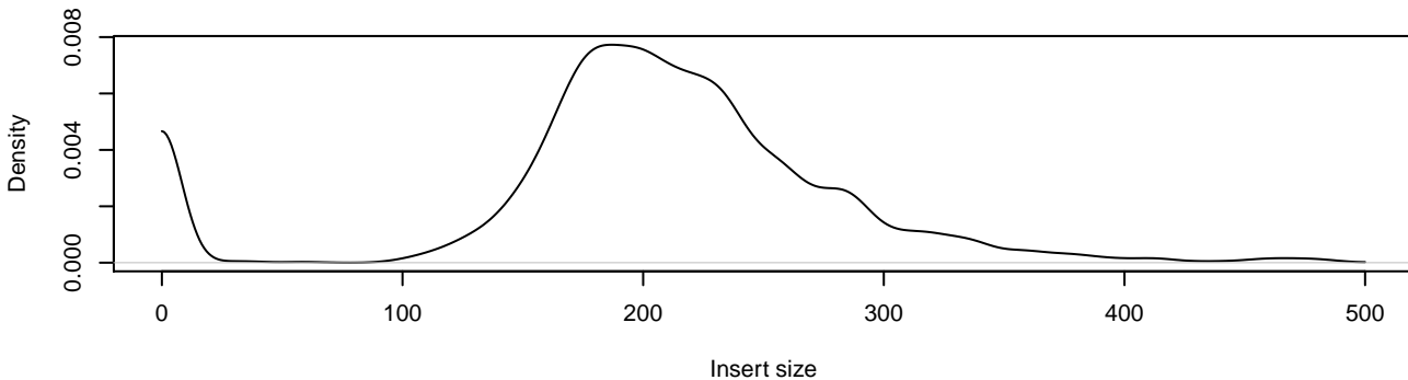
Insert size of reliable breakpoints (distance > 100kb)from = 0 to = 1000
