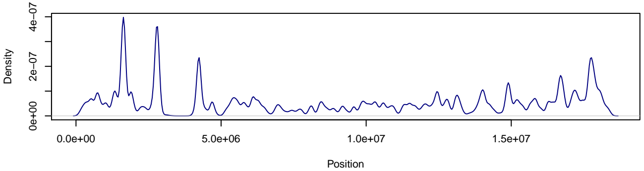
Chromosome 4
