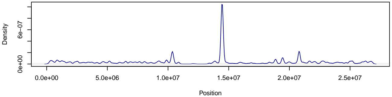
Chromosome 5
