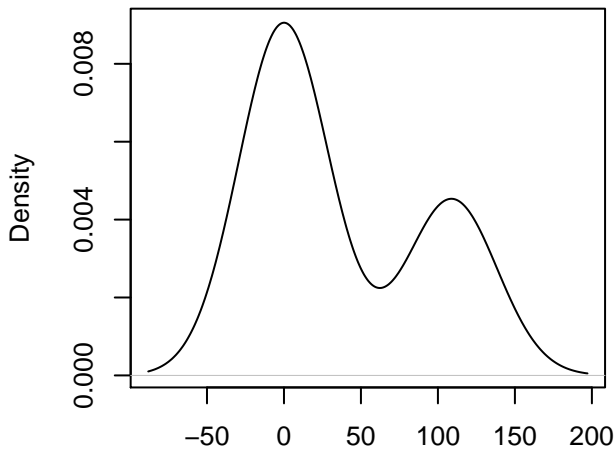
Bp = 90 line = MAGIC.287 , Chr = 5
