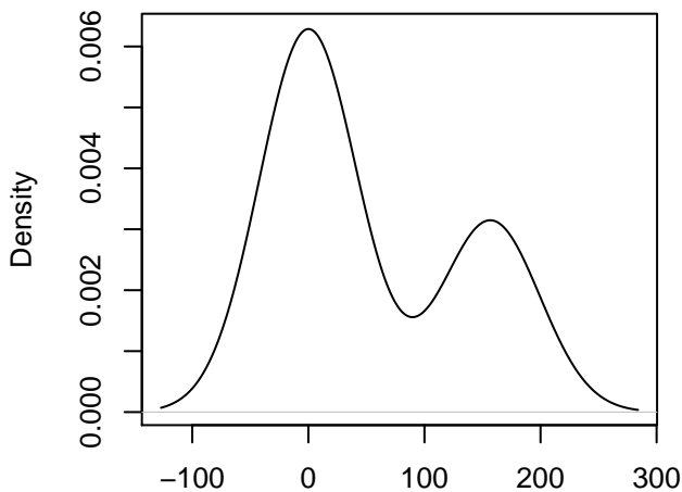
Bp = 91 line = MAGIC.287 , Chr = 5
