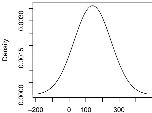
Bp = 4 line = MAGIC.287 , Chr = 1
