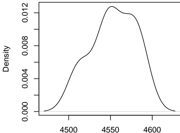
Bp = 73 line = MAGIC.329 , Chr = 3
