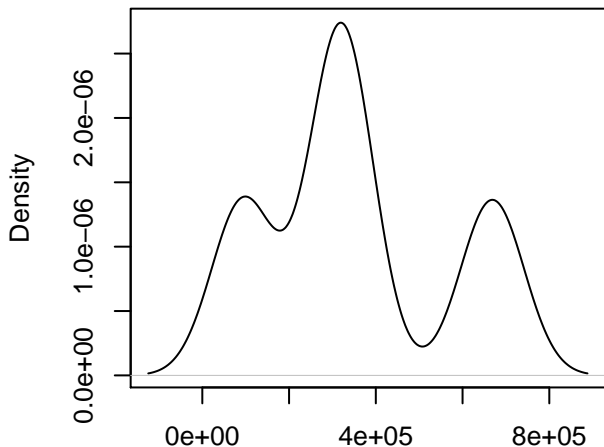
Bp = 79 line = MAGIC.329 , Chr = 3
