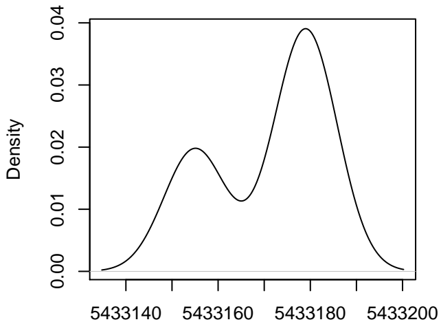
Bp = 11 line = MAGIC.338 , Chr = 1
