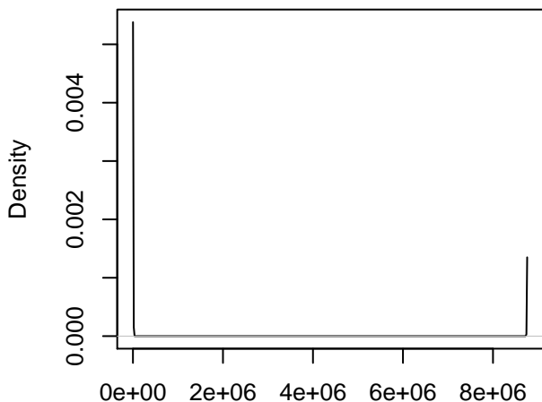
Bp = 36 line = MAGIC.338 , Chr = 2
