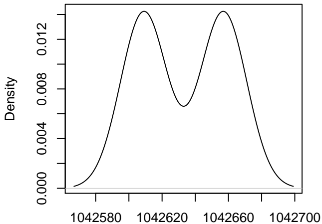
Bp = 7 line = MAGIC.338 , Chr = 1
