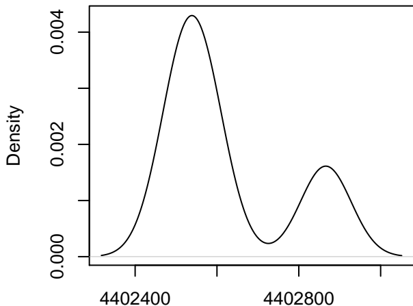
Bp = 25 line = MAGIC.338 , Chr = 2
