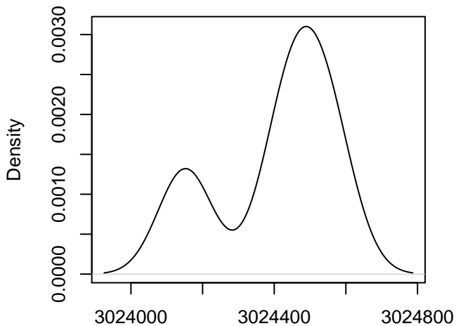
Bp = 19 line = MAGIC.426 , Chr = 1
