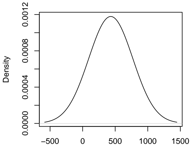
line = MAGIC.105 , Chr = 3
