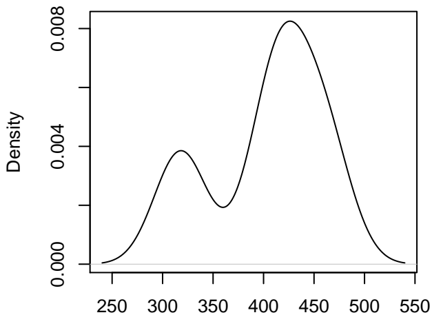
line = MAGIC.149 , Chr = 2
