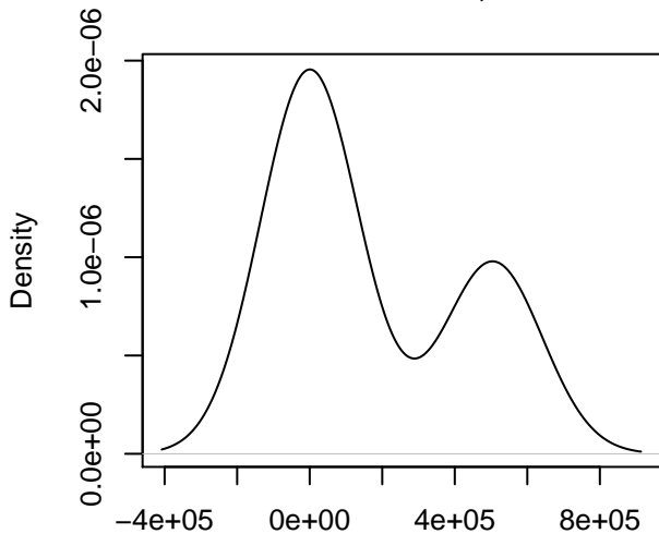
line = MAGIC.149 , Chr = 4
