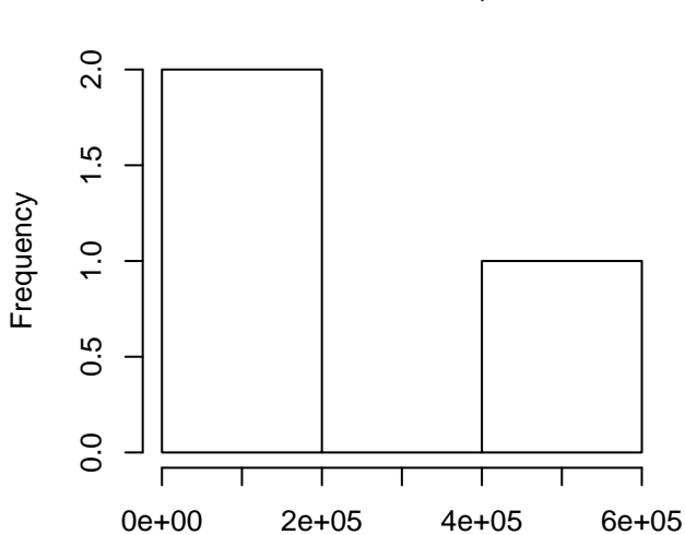
line = MAGIC.149 , Chr = 4
