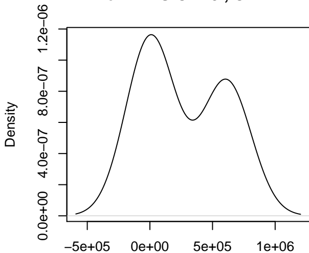
line = MAGIC.149 , Chr = 2
