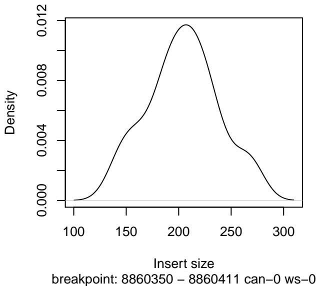
line = MAGIC.175 , Chr = 4
