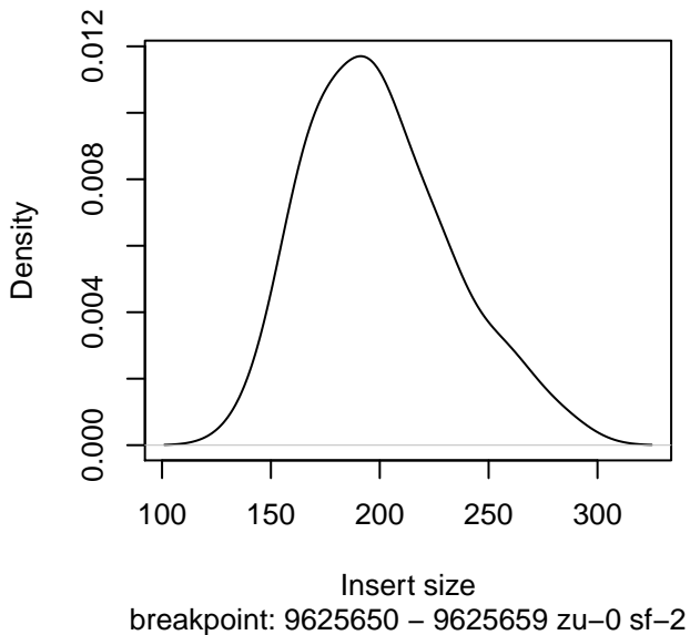
line = MAGIC.175 , Chr = 3
