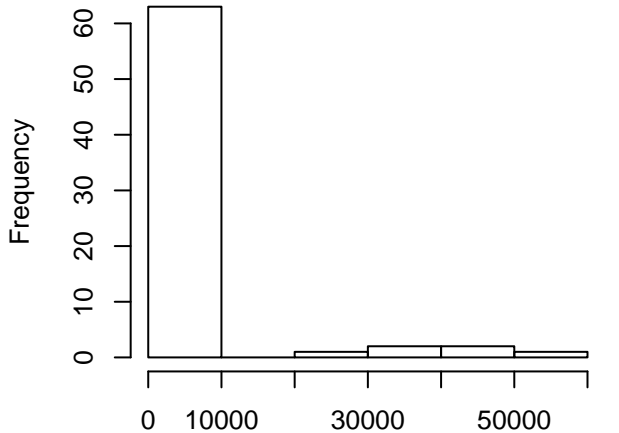
line = MAGIC.433 , Chr = 4
