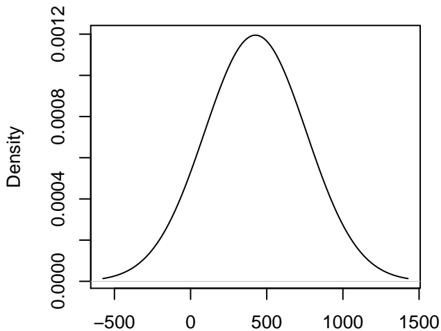
line = MAGIC.433 , Chr = 3
