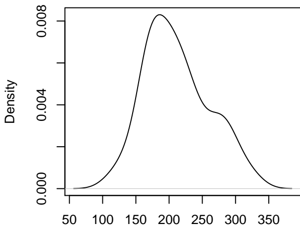
Insert size, N =60 breakpoint: 20199549 – 20199583 tsu-0 rsch-4
