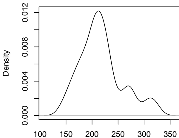
Insert size, N =68 breakpoint: 24175196 – 24175197 rsch-4 mt-0
