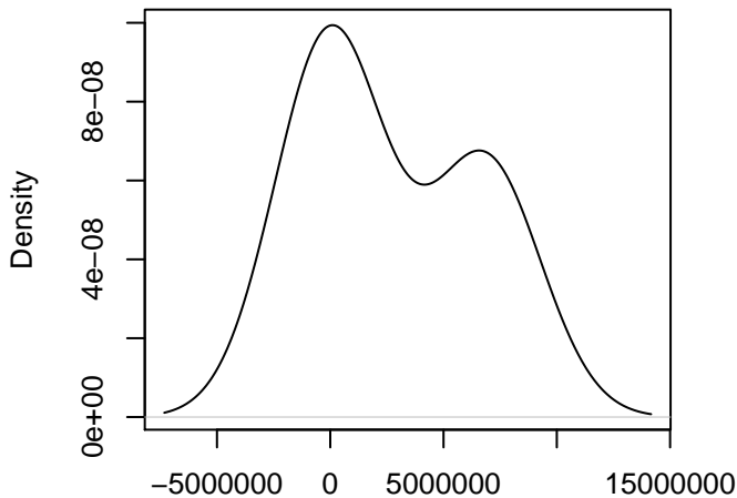
line = MAGIC.183 , Chr = 3
