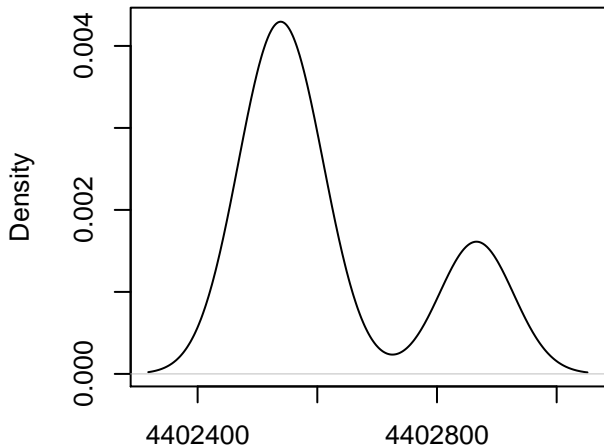
Bp = 18 line = MAGIC.338 , Chr = 2
