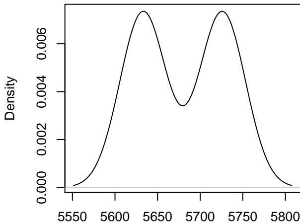
Bp = 23 line = MAGIC.338 , Chr = 2
