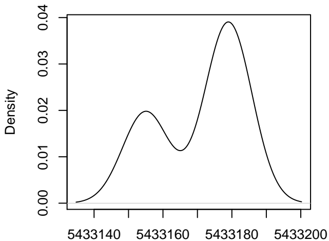
Bp = 8 line = MAGIC.338 , Chr = 1
