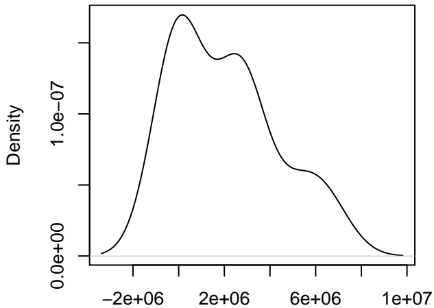
line = MAGIC.105 , Chr = 2
