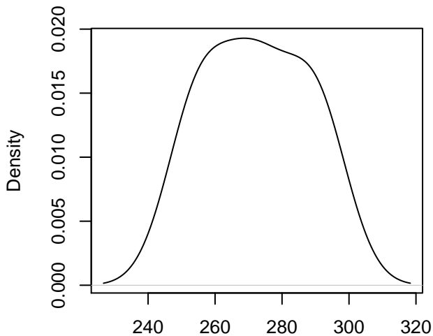
line = MAGIC.105 , Chr = 5
