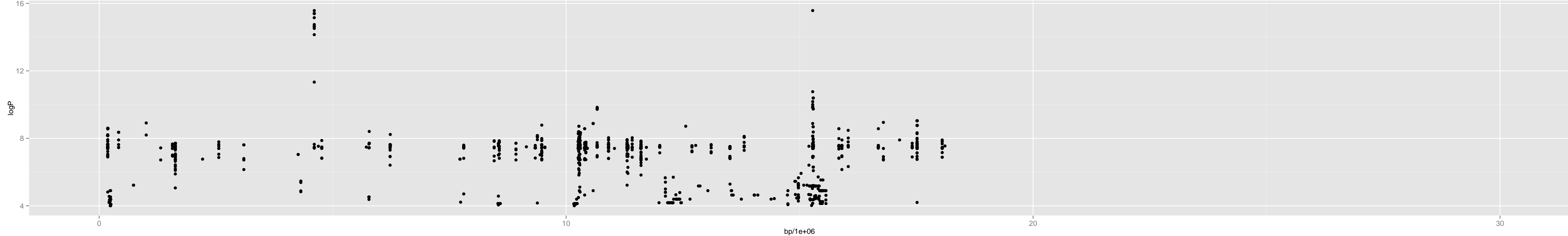
Chromosome 4 – 1_wil.2_18962350_14_13
