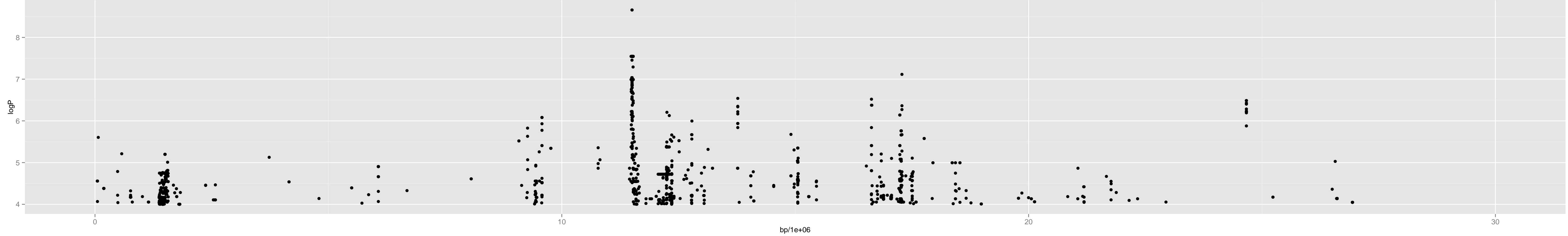
Chromosome 5 – 4_ws.0_4196767_32_28
