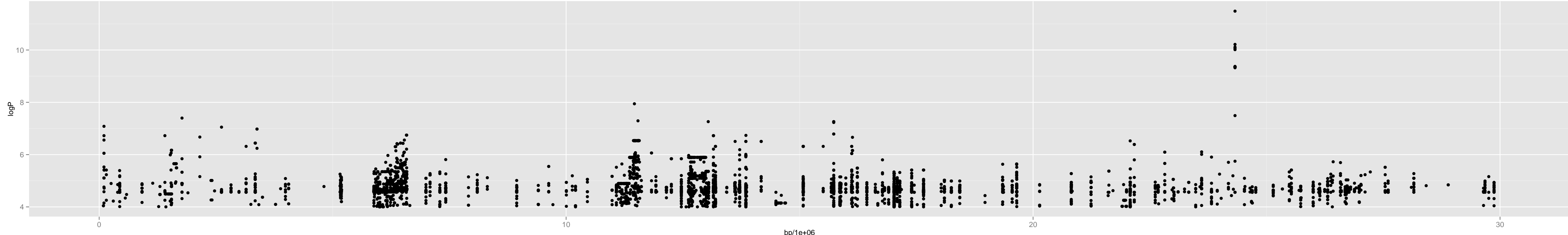
Chromosome 1 – 4_wu.0_2393103_22_8
