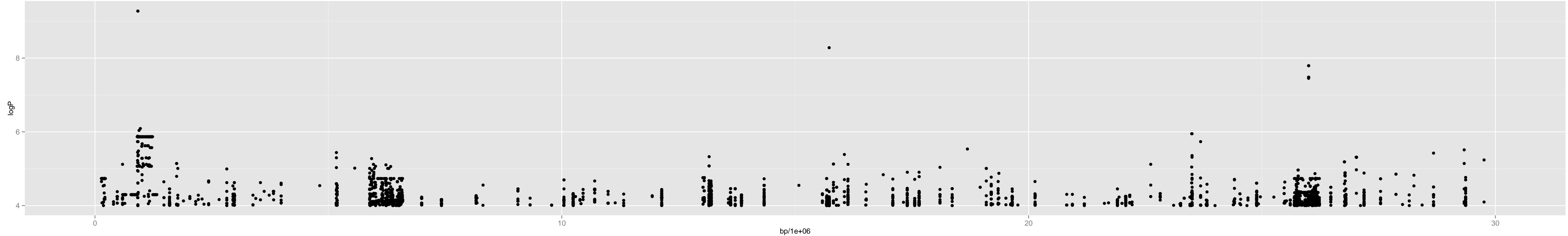
Chromosome 1 – 4_wu.0_4209623_25_25
