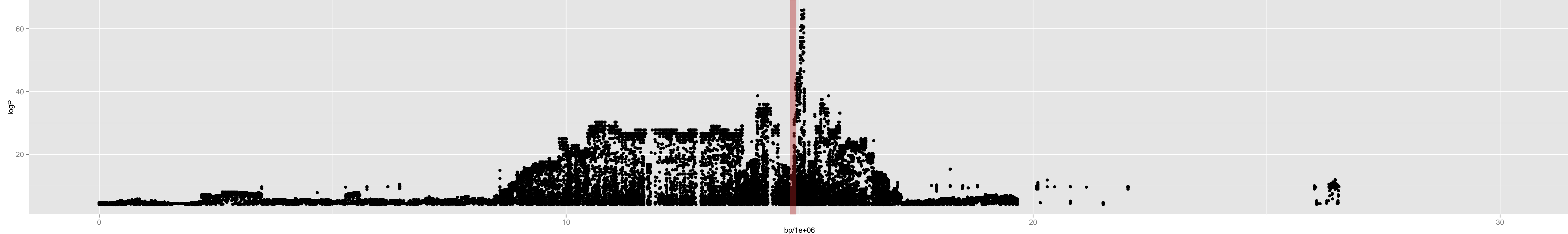
Chromosome 5 – 5_hi.0_14864223_11_2
